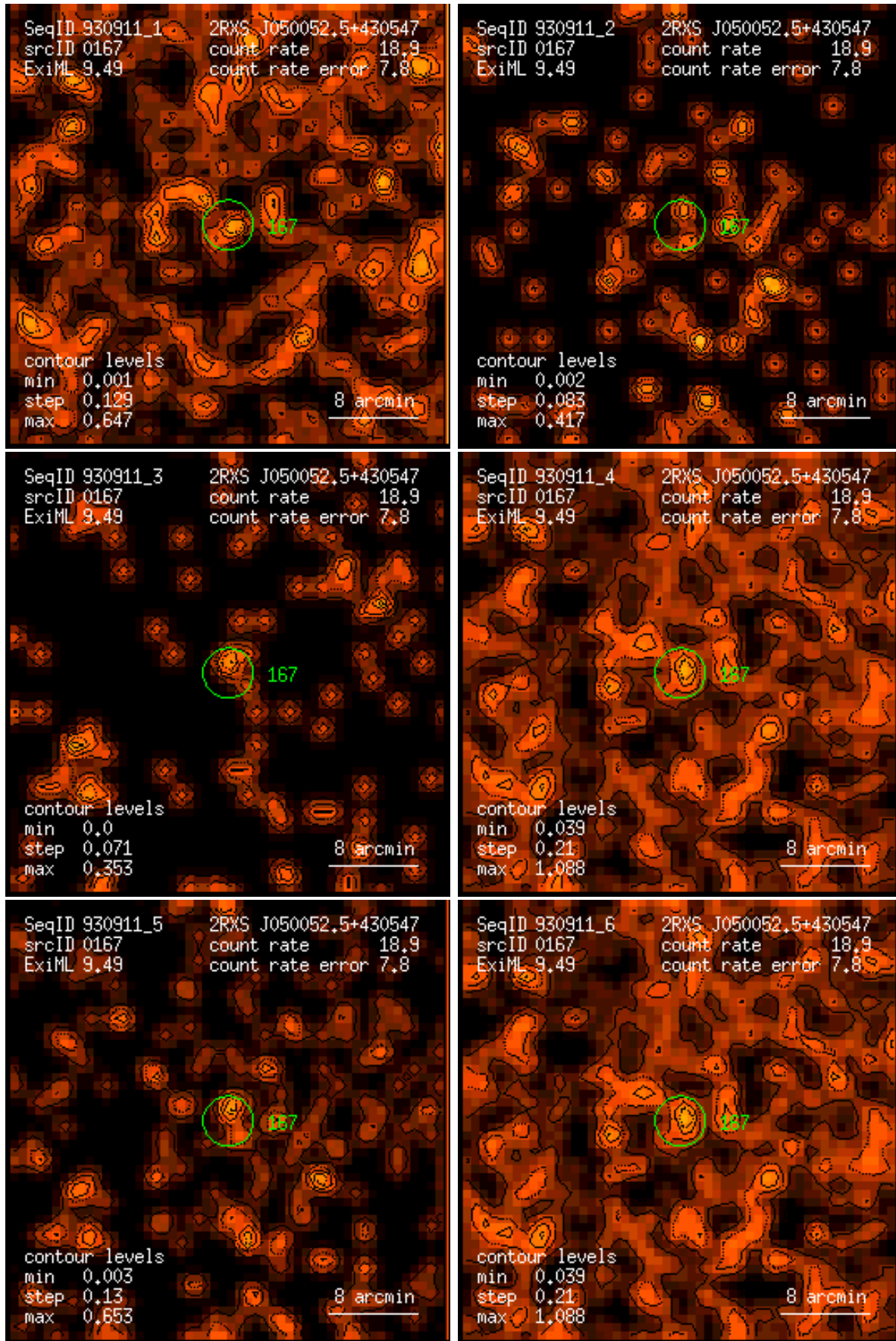
Figure 167: RASS 930911: detection 0167: band rate images, Gaussian filter: (1) PSPC channels 11 – 41, (2) 52 – 90, (3) 91 – 201, (4) 11 – 235, (5) 52 – 201, (6) 11 – 201. Broad band rates in counts/ks. Band rate contour levels in counts/ks/arcmin 2 .
