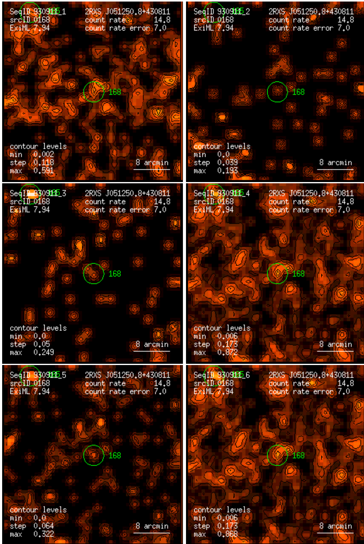
Figure 168: RASS 930911: detection 0168: band rate images, Gaussian filter: (1) PSPC channels 11 – 41, (2) 52 – 90, (3) 91 – 201, (4) 11 – 235, (5) 52 – 201, (6) 11 – 201. Broad band rates in counts/ks. Band rate contour levels in counts/ks/arcmin 2 .
