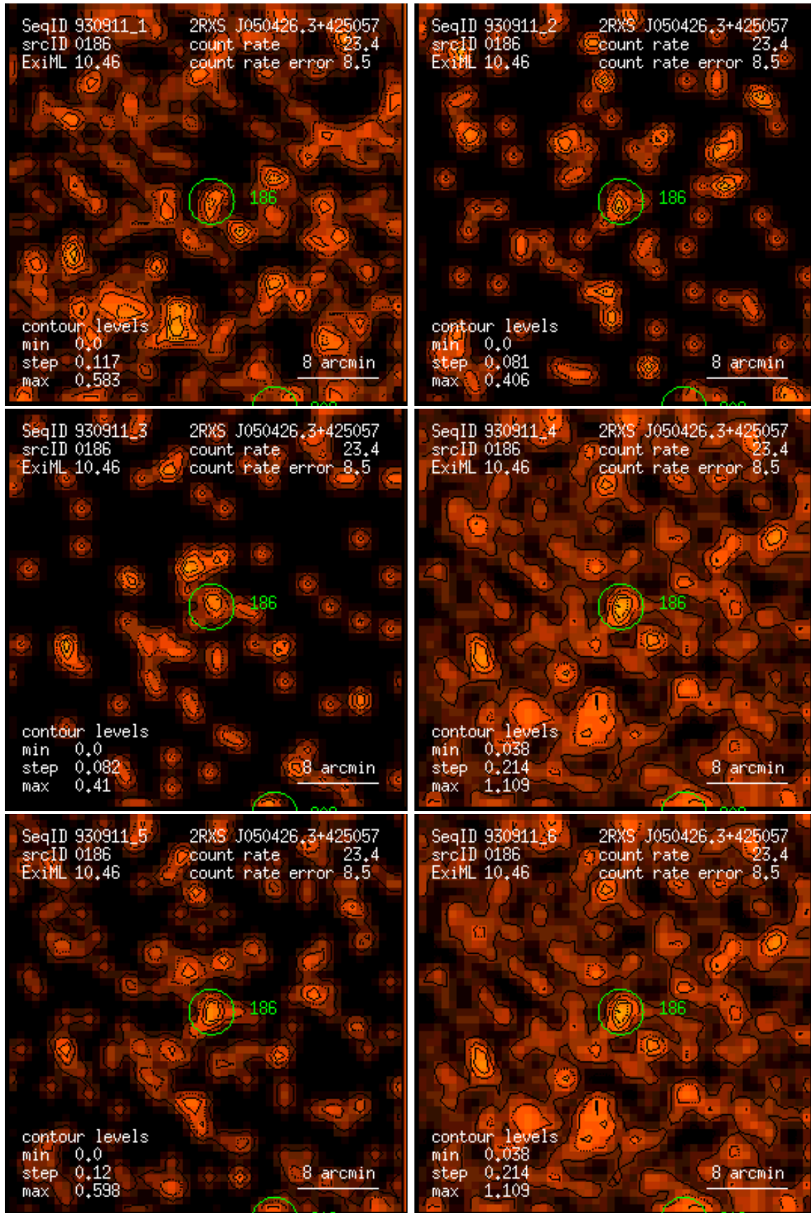
Figure 186: RASS 930911: detection 0186: band rate images, Gaussian filter: (1) PSPPC channels 11 – 41, (2) 52 – 90, (3) 91 – 201, (4) 11 – 235, (5) 52 – 201, (6) 11 – 201. Broad band rates in counts/ks. Band rate contour levels in counts/ks/arcmin 2 .
