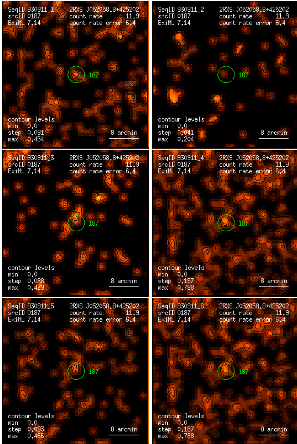
Figure 187: RASS 930911: detection 0187: band rate images, Gaussian filter: (1) PSPC channels 11 – 41, (2) 52 – 90, (3) 91 – 201, (4) 11 – 235, (5) 52 – 201, (6) 11 – 201. Broad band rates in counts/ks. Band rate contour levels in counts/ks/arcmin 2 .
