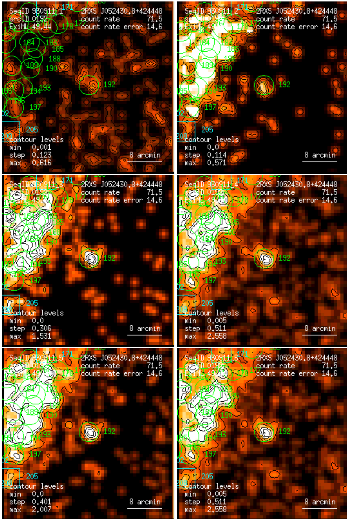
Figure 192: RASS 930911: detection 0192: band rate images, Gaussian filter: (1) PSPC channels 11 – 41, (2) 52 – 90, (3) 91 – 201, (4) 11 – 235, (5) 52 – 201, (6) 11 – 201. Broad band rates in counts/ks. Band rate contour levels in counts/ks/arcmin 2 .
