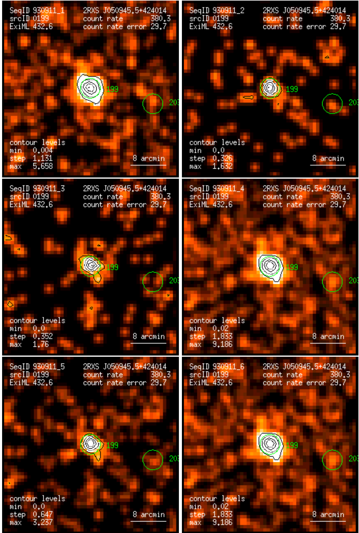
Figure 199: RASS 930911: detection 0199: band rate images, Gaussian filter: (1) PSPC channels 11 – 41, (2) 52 – 90, (3) 91 – 201, (4) 11 – 235, (5) 52 – 201, (6) 11 – 201. Broad band rates in counts/ks. Band rate contour levels in counts/ks/arcmin 2 .
