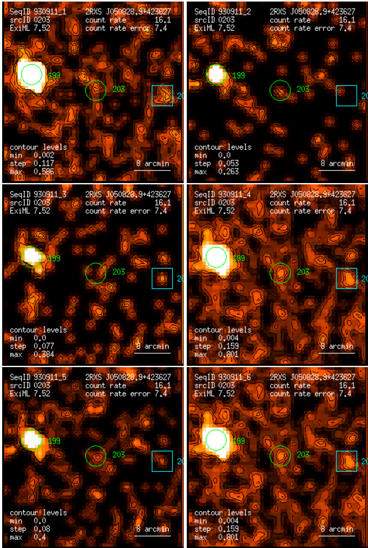
Figure 203: RASS 930911: detection 0203: band rate images, Gaussian filter: (1) PSPC channels 11 – 41, (2) 52 – 90, (3) 91 – 201, (4) 11 – 235, (5) 52 – 201, (6) 11 – 201. Broad band rates in counts/ks. Band rate contour levels in counts/ks/arcmin 2 .
