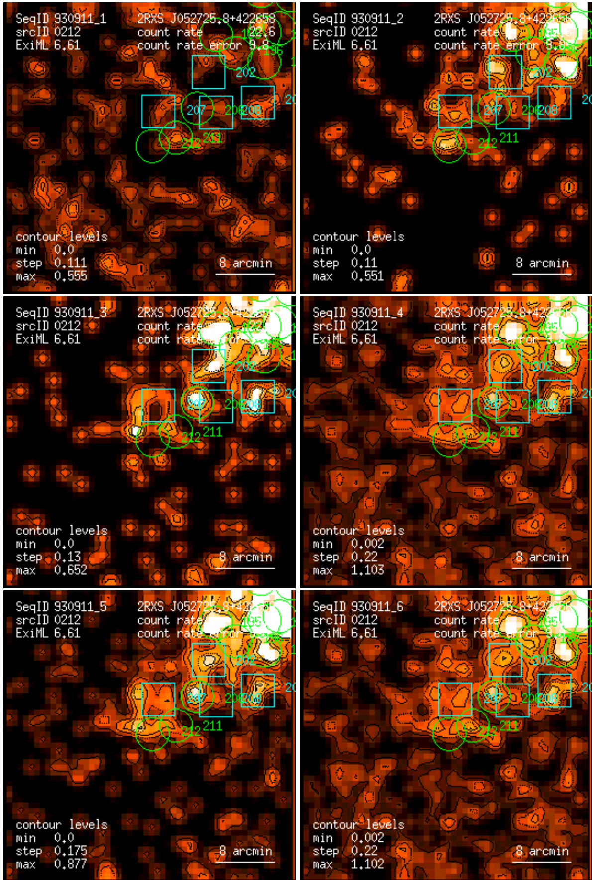
Figure 212: RASS 930911: detection 0212: band rate images, Gaussian filter: (1) PSPC channels 11 – 41, (2) 52 – 90, (3) 91 – 201, (4) 11 – 235, (5) 52 – 201, (6) 11 – 201. Broad band rates in counts/ks. Band rate contour levels in counts/ks/arcmin 2 .
