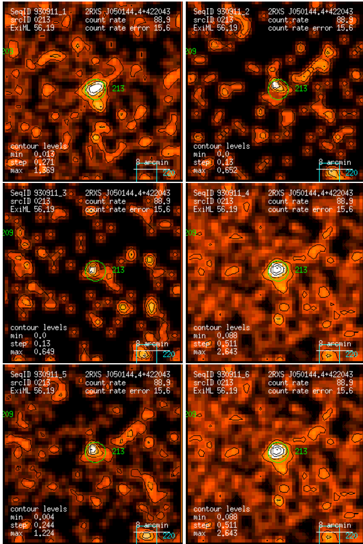
Figure 213: RASS 930911: detection 0213: band rate images, Gaussian filter: (1) PSPC channels 11 – 41, (2) 52 – 90, (3) 91 – 201, (4) 11 – 235, (5) 52 – 201, (6) 11 – 201. Broad band rates in counts/ks. Band rate contour levels in counts/ks/arcmin 2 .
