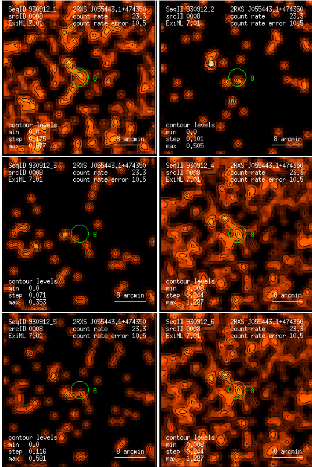
Figure 8: RASS 930912: detection 0008: band rate images, Gaussian filter: (1) PSPC channels 11 – 41, (2) 52 – 90, (3) 91 – 201, (4) 11 – 235, (5) 52 – 201, (6) 11 – 201. Broad band rates in counts/ks. Band rate contour levels in counts/ks/arcmin 2 .
