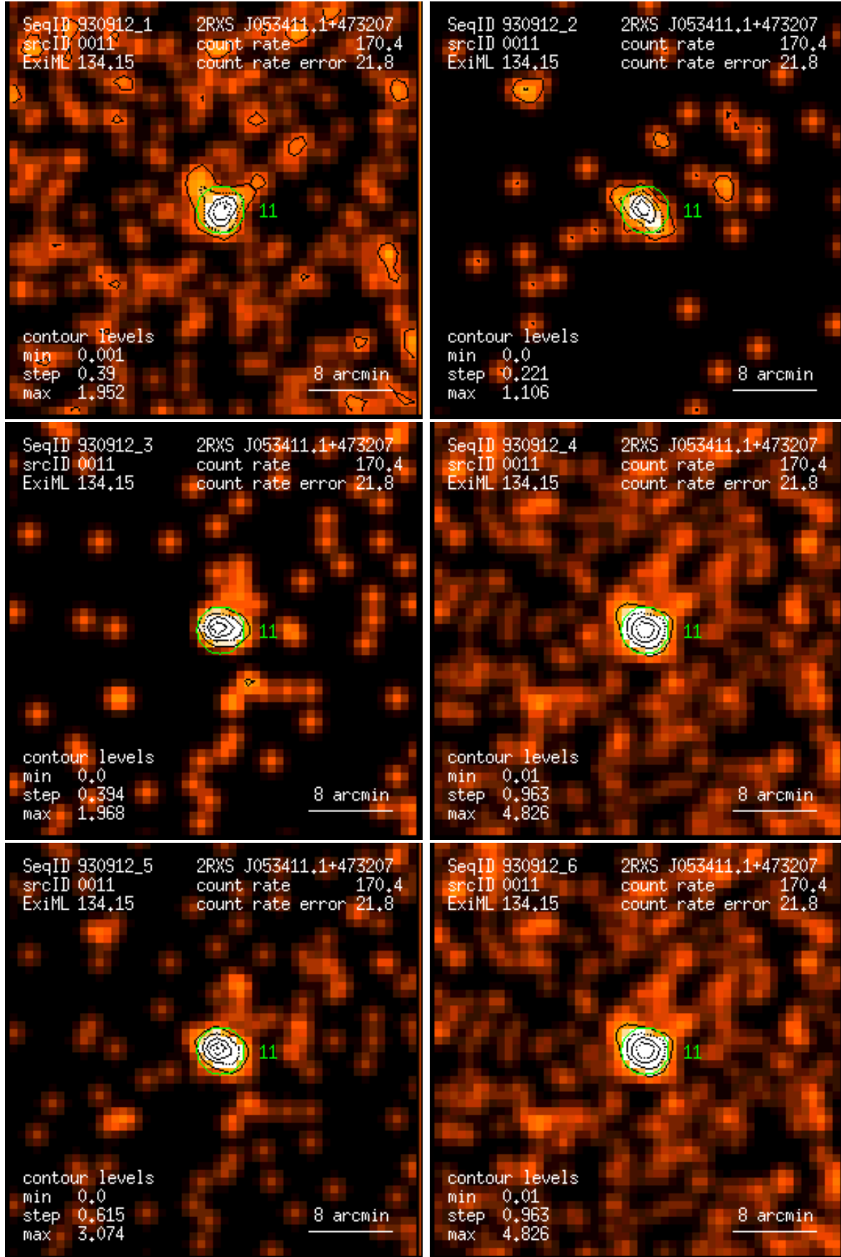
Figure 11: RASS 930912: detection 0011: band rate images, Gaussian filter: (1) PSPC channels 11 – 41, (2) 52 – 90, (3) 91 – 201, (4) 11 – 235, (5) 52 – 201, (6) 11 – 201. Broad band rates in counts/ks. Band rate contour levels in counts/ks/arcmin 2 .
