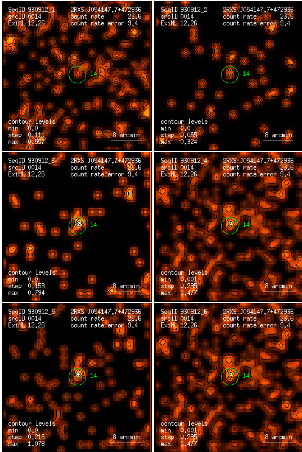
Figure 14: RASS 930912: detection 0014: band rate images, Gaussian filter: (1) PSPC channels 11 – 41, (2) 52 – 90, (3) 91 – 201, (4) 11 – 235, (5) 52 – 201, (6) 11 – 201. Broad band rates in counts/ks. Band rate contour levels in counts/ks/arcmin 2 .
