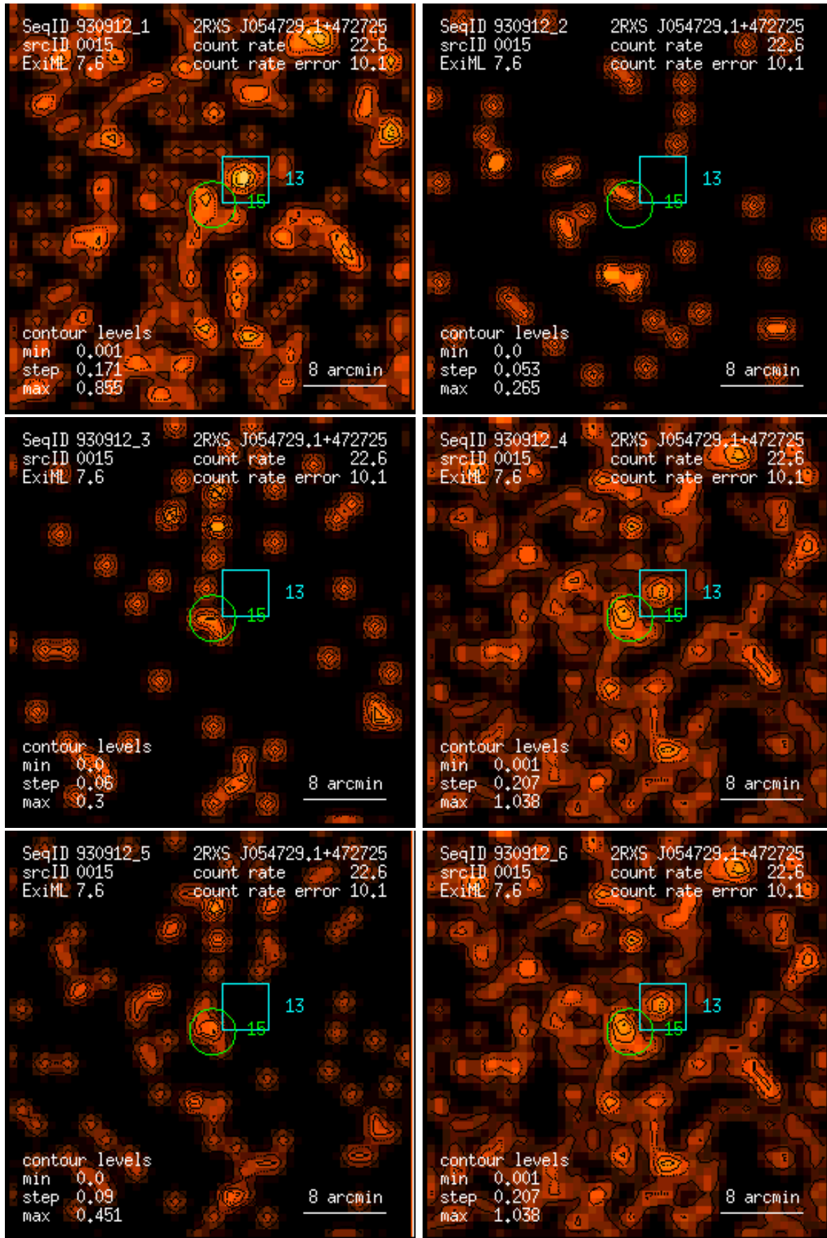
Figure 15: RASS 930912: detection 0015: band rate images, Gaussian filter: (1) PSPC channels 11 – 41, (2) 52 – 90, (3) 91 – 201, (4) 11 – 235, (5) 52 – 201, (6) 11 – 201. Broad band rates in counts/ks. Band rate contour levels in counts/ks/arcmin 2 .
