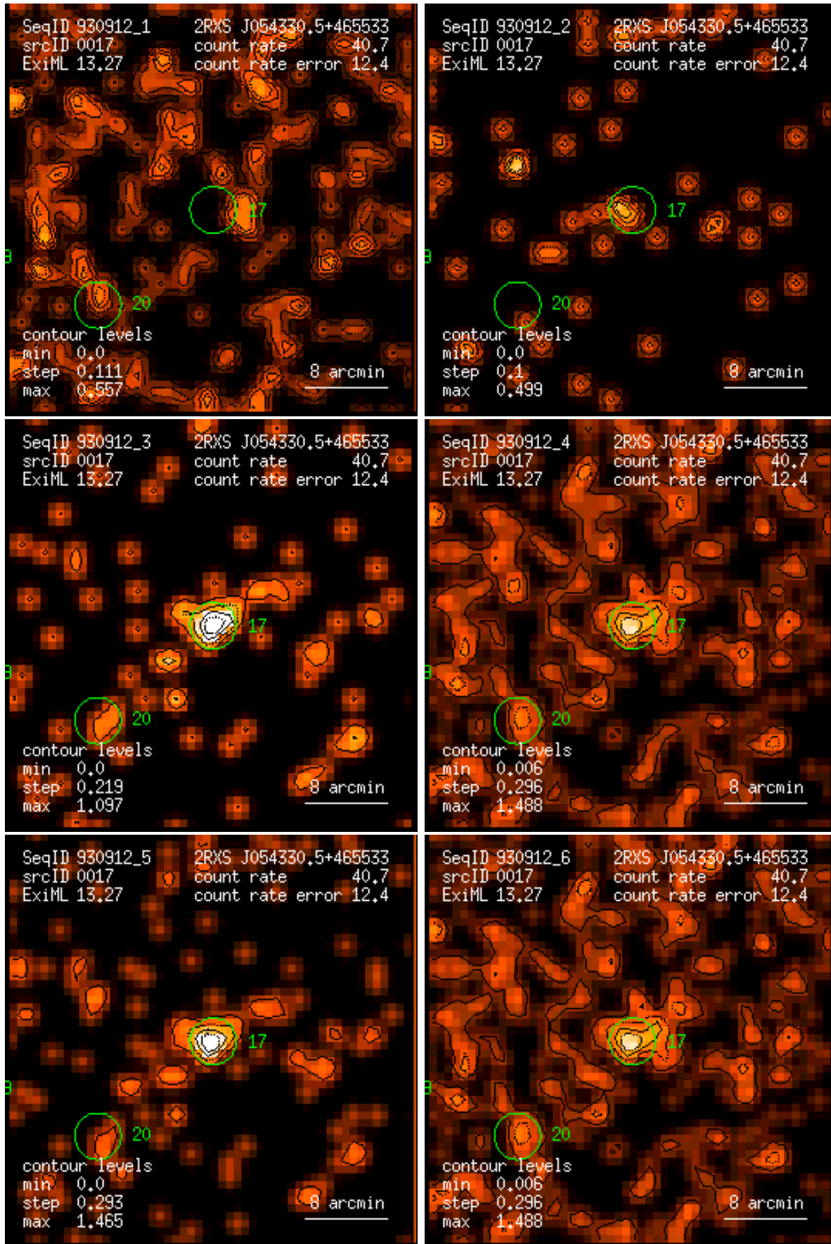
Figure 17: RASS 930912: detection 0017: band rate images, Gaussian filter: (1) PSPC channels 11 – 41, (2) 52 – 90, (3) 91 – 201, (4) 11 – 235, (5) 52 – 201, (6) 11 – 201. Broad band rates in counts/ks. Band rate contour levels in counts/ks/arcmin 2 .
