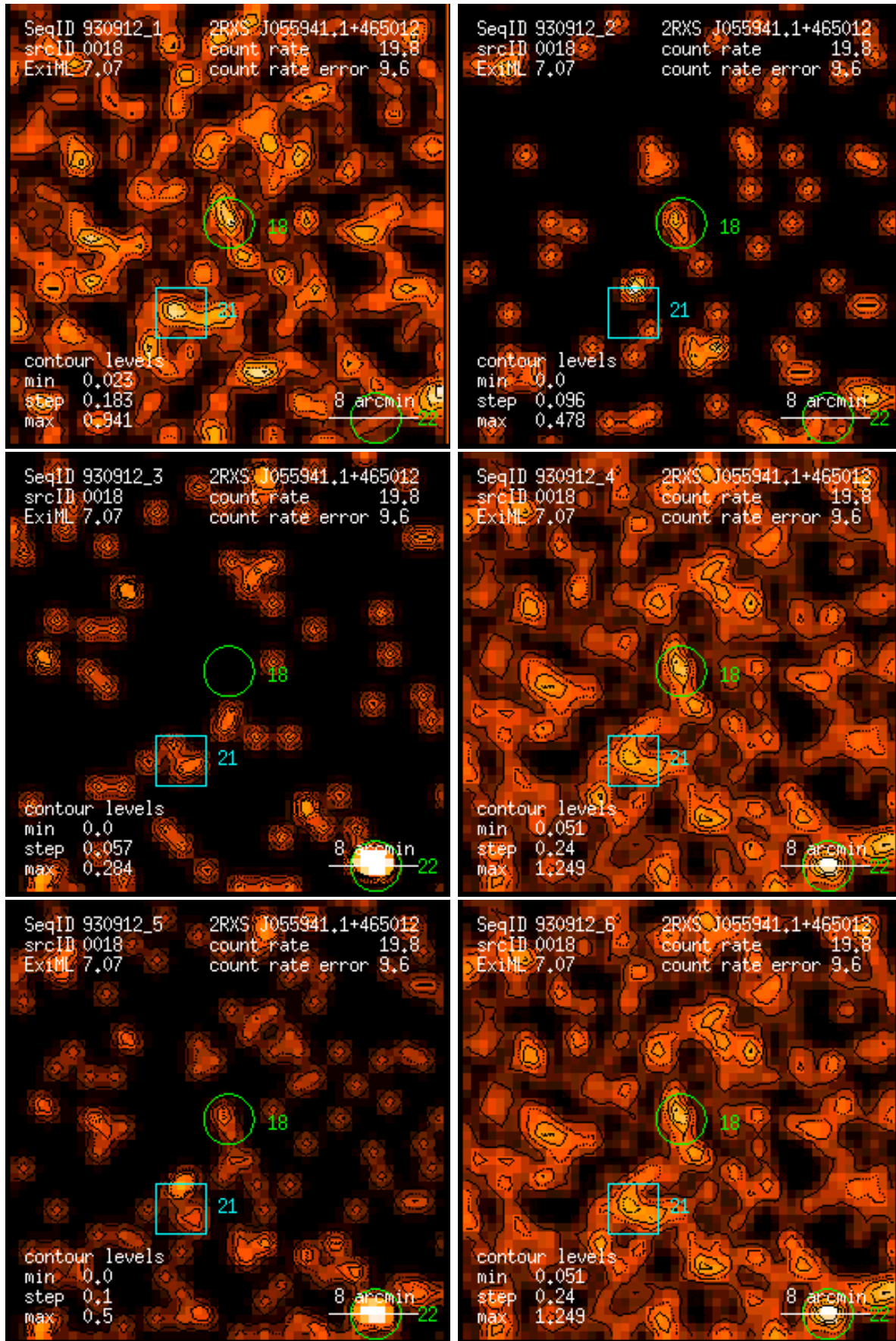
Figure 18: RASS 930912: detection 0018: band rate images, Gaussian filter: (1) PSPC channels 11 – 41, (2) 52 – 90, (3) 91 – 201, (4) 11 – 235, (5) 52 – 201, (6) 11 – 201. Broad band rates in counts/ks. Band rate contour levels in counts/ks/arcmin 2 .
