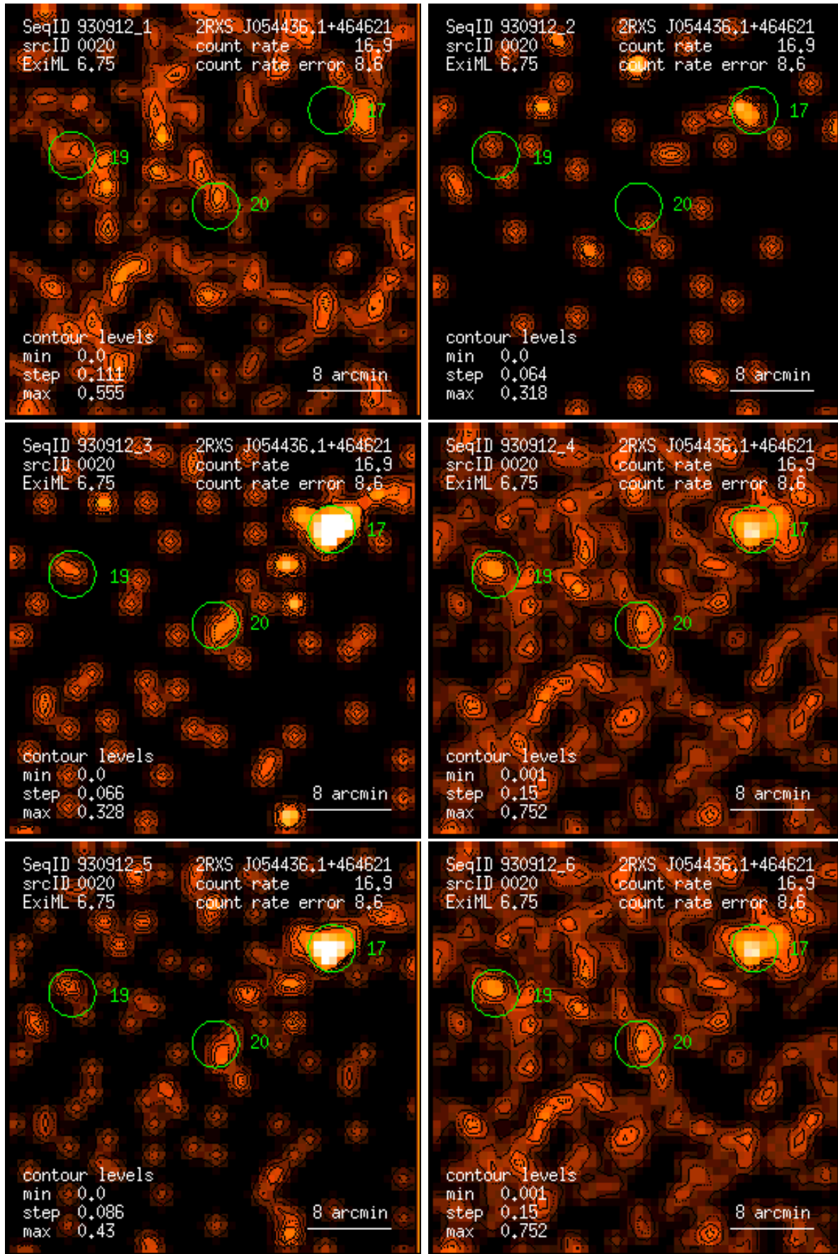
Figure 20: RASS 930912: detection 0020: band rate images, Gaussian filter: (1) PSPC channels 11 – 41, (2) 52 – 90, (3) 91 – 201, (4) 11 – 235, (5) 52 – 201, (6) 11 – 201. Broad band rates in counts/ks. Band rate contour levels in counts/ks/arcmin 2 .
