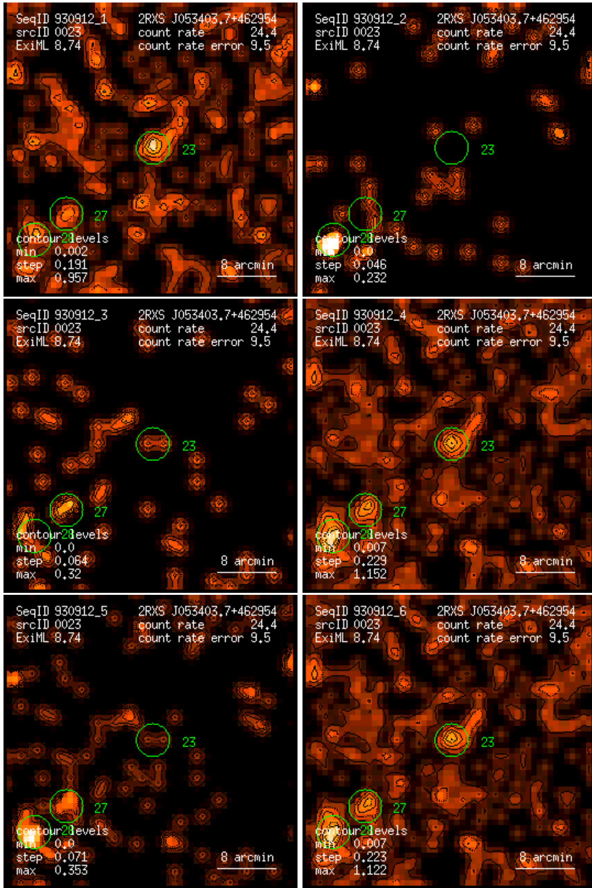
Figure 23: RASS 930912: detection 0023: band rate images, Gaussian filter: (1) PSPC channels 11 – 41, (2) 52 – 90, (3) 91 – 201, (4) 11 – 235, (5) 52 – 201, (6) 11 – 201. Broad band rates in counts/ks. Band rate contour levels in counts/ks/arcmin 2 .
