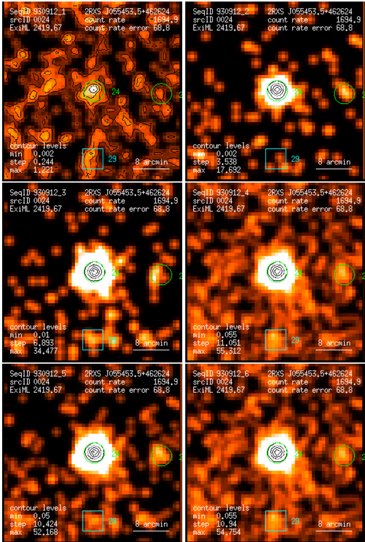
Figure 24: RASS 930912: detection 0024: band rate images, Gaussian filter: (1) PSPC channels 11 – 41, (2) 52 – 90, (3) 91 – 201, (4) 11 – 235, (5) 52 – 201, (6) 11 – 201. Broad band rates in counts/ks. Band rate contour levels in counts/ks/arcmin 2 .
