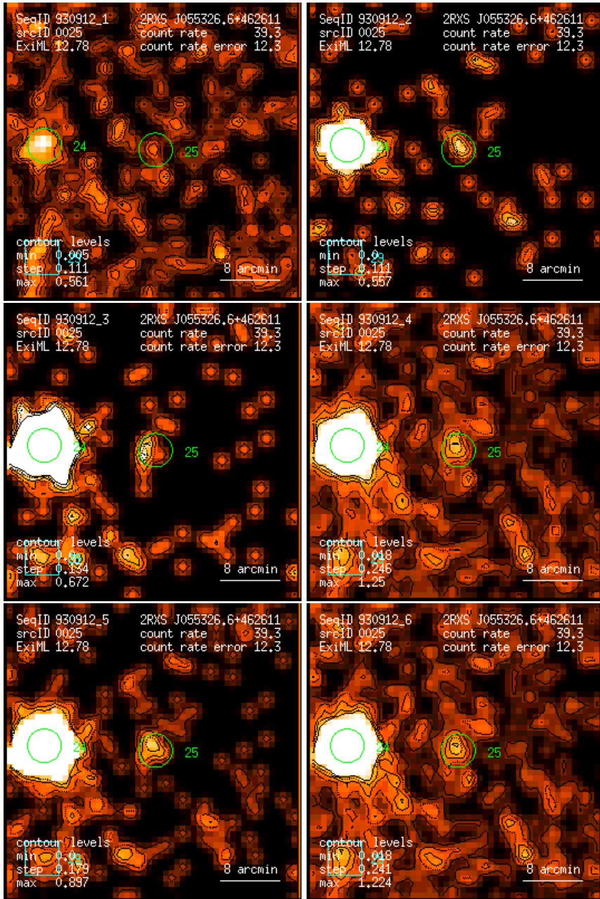
Figure 25: RASS 930912: detection 0025: band rate images, Gaussian filter: (1) PSPC channels 11 – 41, (2) 52 – 90, (3) 91 – 201, (4) 11 – 235, (5) 52 – 201, (6) 11 – 201. Broad band rates in counts/ks. Band rate contour levels in counts/ks/arcmin 2 .
