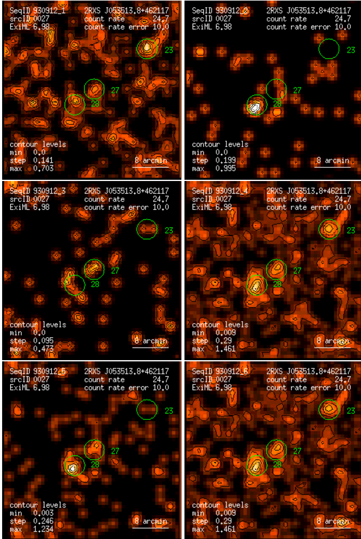
Figure 27: RASS 930912: detection 0027: band rate images, Gaussian filter: (1) PSPC channels 11 – 41, (2) 52 – 90, (3) 91 – 201, (4) 11 – 235, (5) 52 – 201, (6) 11 – 201. Broad band rates in counts/ks. Band rate contour levels in counts/ks/arcmin 2 .
