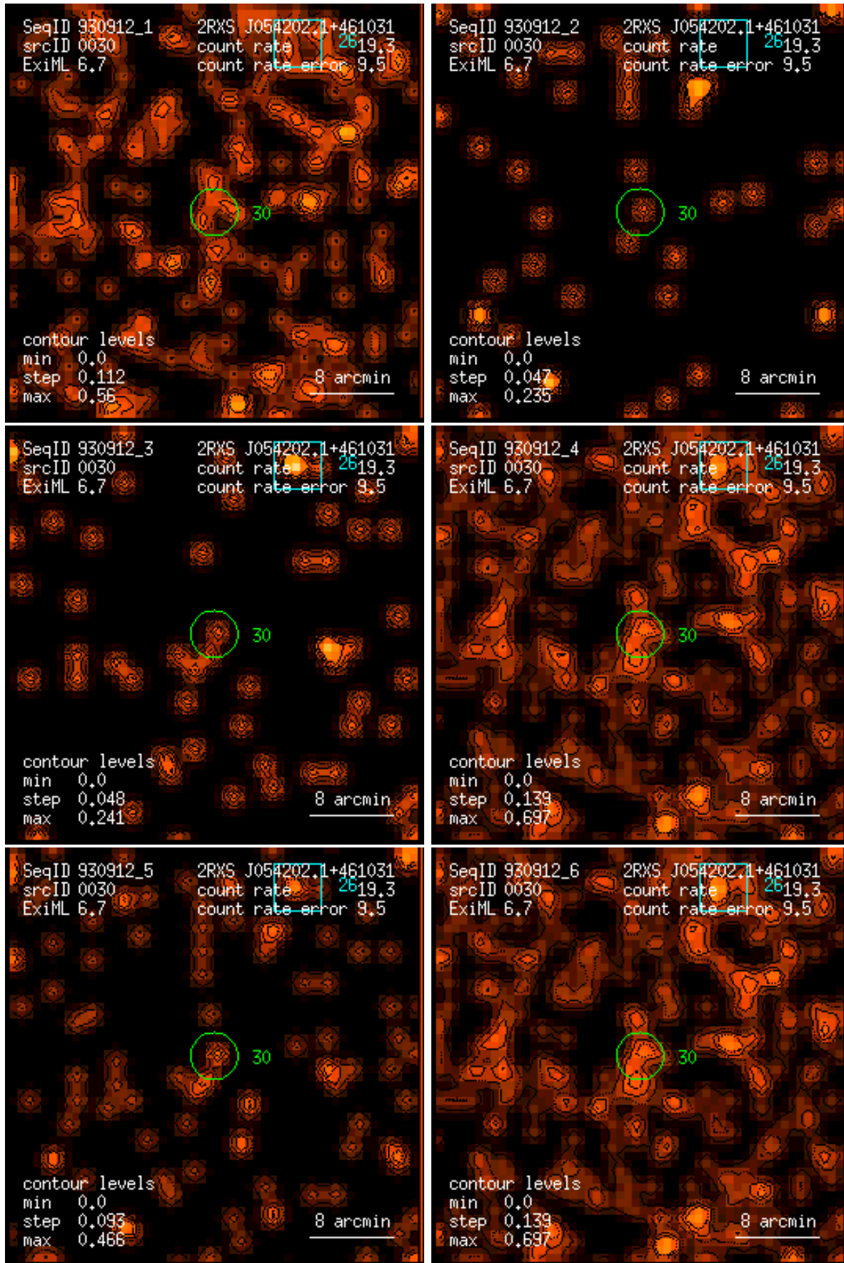
Figure 30: RASS 930912: detection 0030: band rate images, Gaussian filter: (1) PSPC channels 11 – 41, (2) 52 – 90, (3) 91 – 201, (4) 11 – 235, (5) 52 – 201, (6) 11 – 201. Broad band rates in counts/ks. Band rate contour levels in counts/ks/arcmin 2 .
