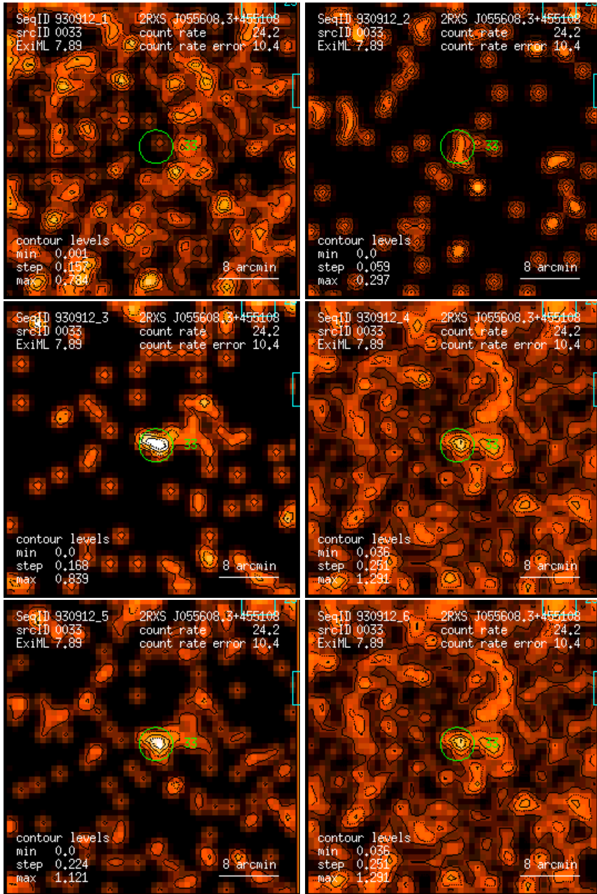
Figure 33: RASS 930912: detection 0033: band rate images, Gaussian filter: (1) PSPC channels 11 – 41, (2) 52 – 90, (3) 91 – 201, (4) 11 – 235, (5) 52 – 201, (6) 11 – 201. Broad band rates in counts/ks. Band rate contour levels in counts/ks/arcmin 2 .
