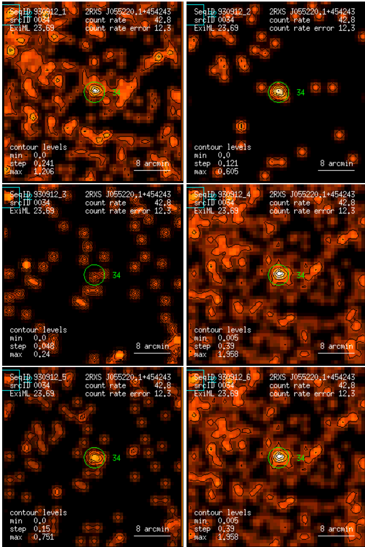
Figure 34: RASS 930912: detection 0034: band rate images, Gaussian filter: (1) PSPC channels 11 – 41, (2) 52 – 90, (3) 91 – 201, (4) 11 – 235, (5) 52 – 201, (6) 11 – 201. Broad band rates in counts/ks. Band rate contour levels in counts/ks/arcmin 2 .
