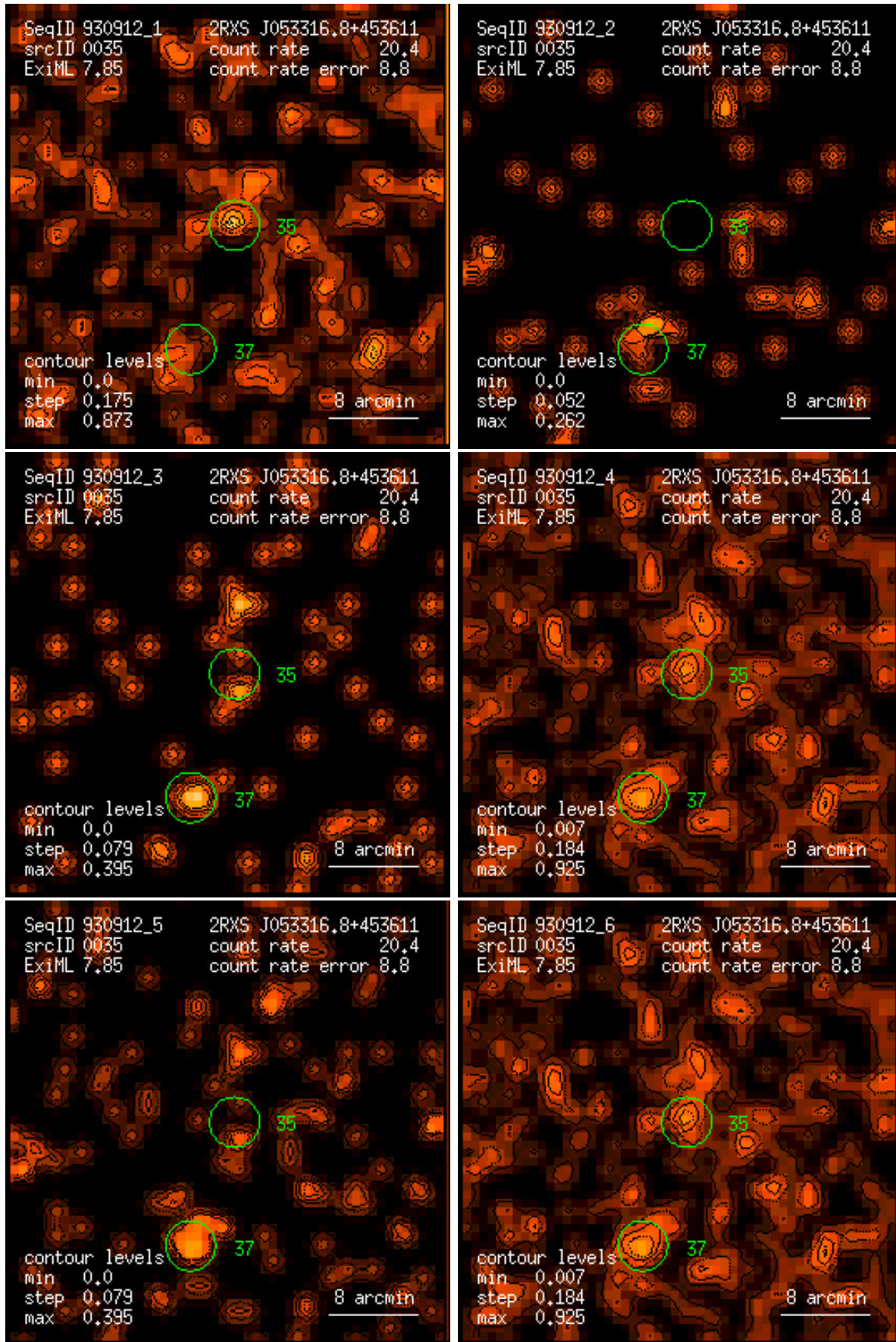
Figure 35: RASS 930912: detection 0035: band rate images, Gaussian filter: (1) PSPC channels 11 – 41, (2) 52 – 90, (3) 91 – 201, (4) 11 – 235, (5) 52 – 201, (6) 11 – 201. Broad band rates in counts/ks. Band rate contour levels in counts/ks/arcmin 2 .
