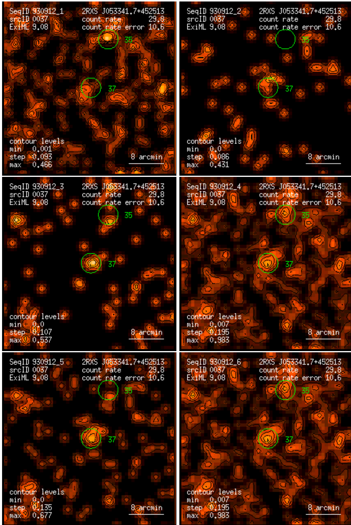
Figure 37: RASS 930912: detection 0037: band rate images, Gaussian filter: (1) PSPC channels 11 – 41, (2) 52 – 90, (3) 91 – 201, (4) 11 – 235, (5) 52 – 201, (6) 11 – 201. Broad band rates in counts/ks. Band rate contour levels in counts/ks/arcmin 2 .
