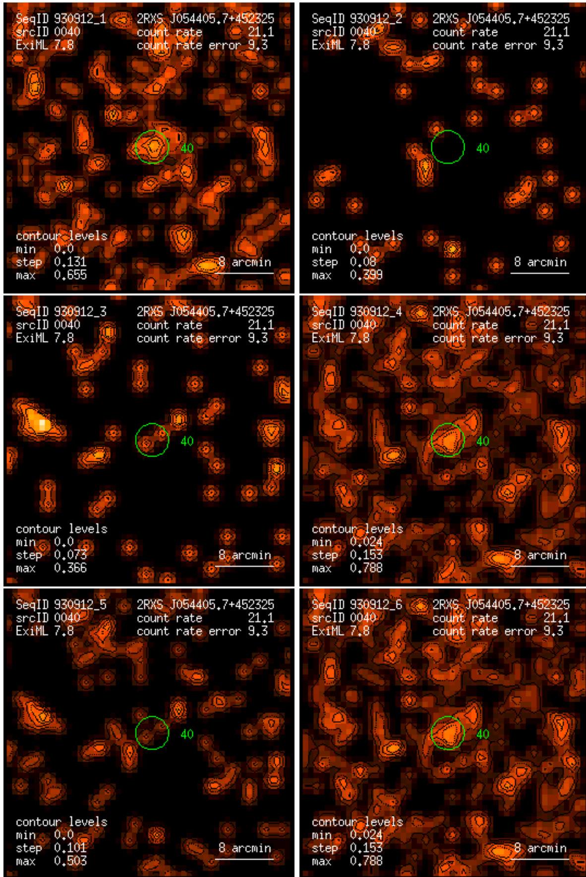
Figure 40: RASS 930912: detection 0040: band rate images, Gaussian filter: (1) PSPC channels 11 – 41, (2) 52 – 90, (3) 91 – 201, (4) 11 – 235, (5) 52 – 201, (6) 11 – 201. Broad band rates in counts/ks. Band rate contour levels in counts/ks/arcmin 2 .
