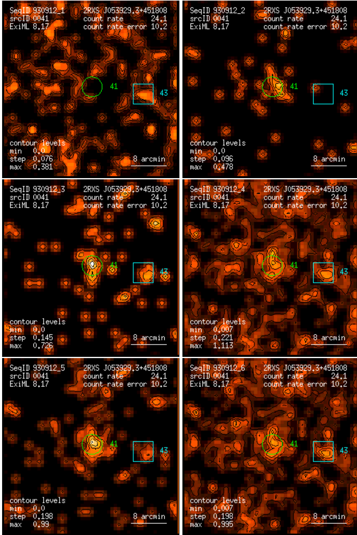
Figure 41: RASS 930912: detection 0041: band rate images, Gaussian filter: (1) PSPC channels 11 – 41, (2) 52 – 90, (3) 91 – 201, (4) 11 – 235, (5) 52 – 201, (6) 11 – 201. Broad band rates in counts/ks. Band rate contour levels in counts/ks/arcmin 2 .
