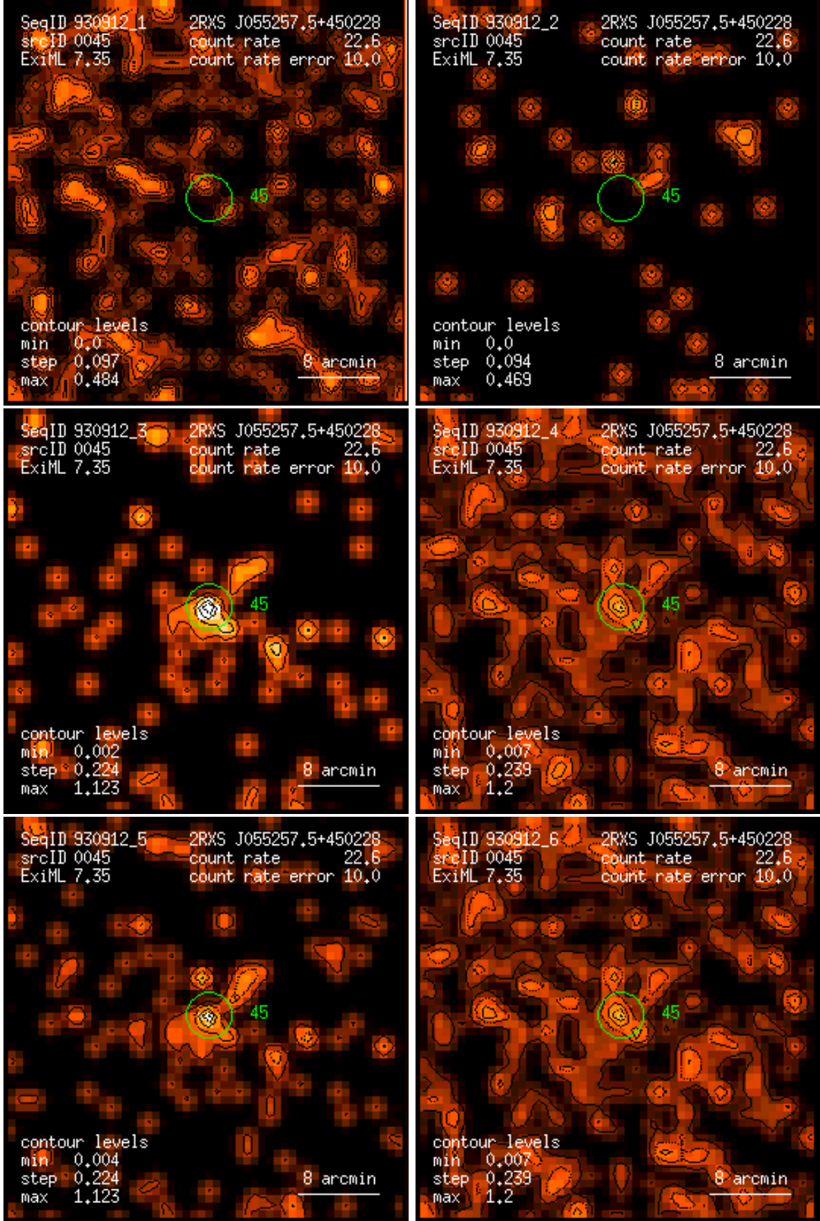
Figure 45: RASS 930912: detection 0045: band rate images, Gaussian filter: (1) PSPC channels 11 – 41, (2) 52 – 90, (3) 91 – 201, (4) 11 – 235, (5) 52 – 201, (6) 11 – 201. Broad band rates in counts/ks. Band rate contour levels in counts/ks/arcmin 2 .
