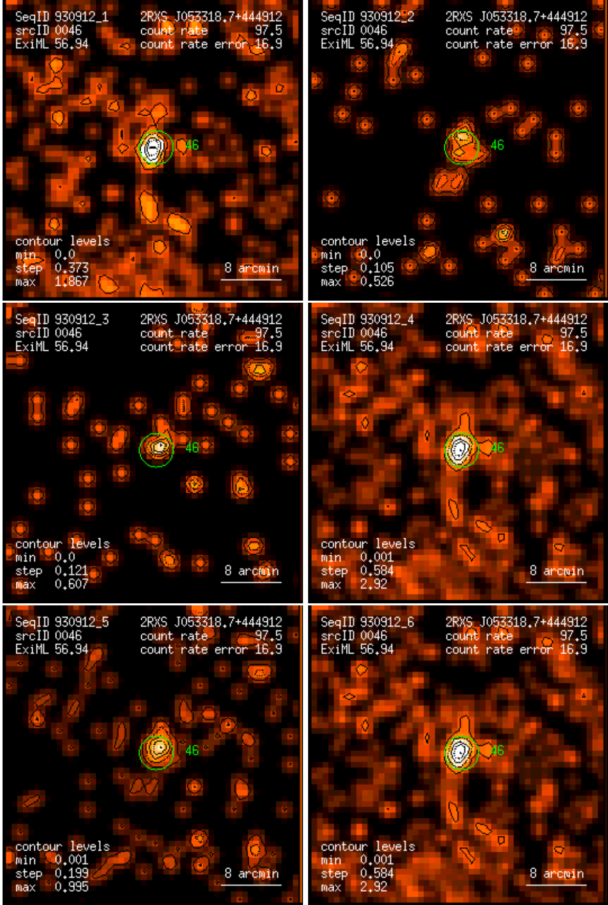
Figure 46: RASS 930912: detection 0046: band rate images, Gaussian filter: (1) PSPC channels 11 – 41, (2) 52 – 90, (3) 91 – 201, (4) 11 – 235, (5) 52 – 201, (6) 11 – 201. Broad band rates in counts/ks. Band rate contour levels in counts/ks/arcmin 2 .
