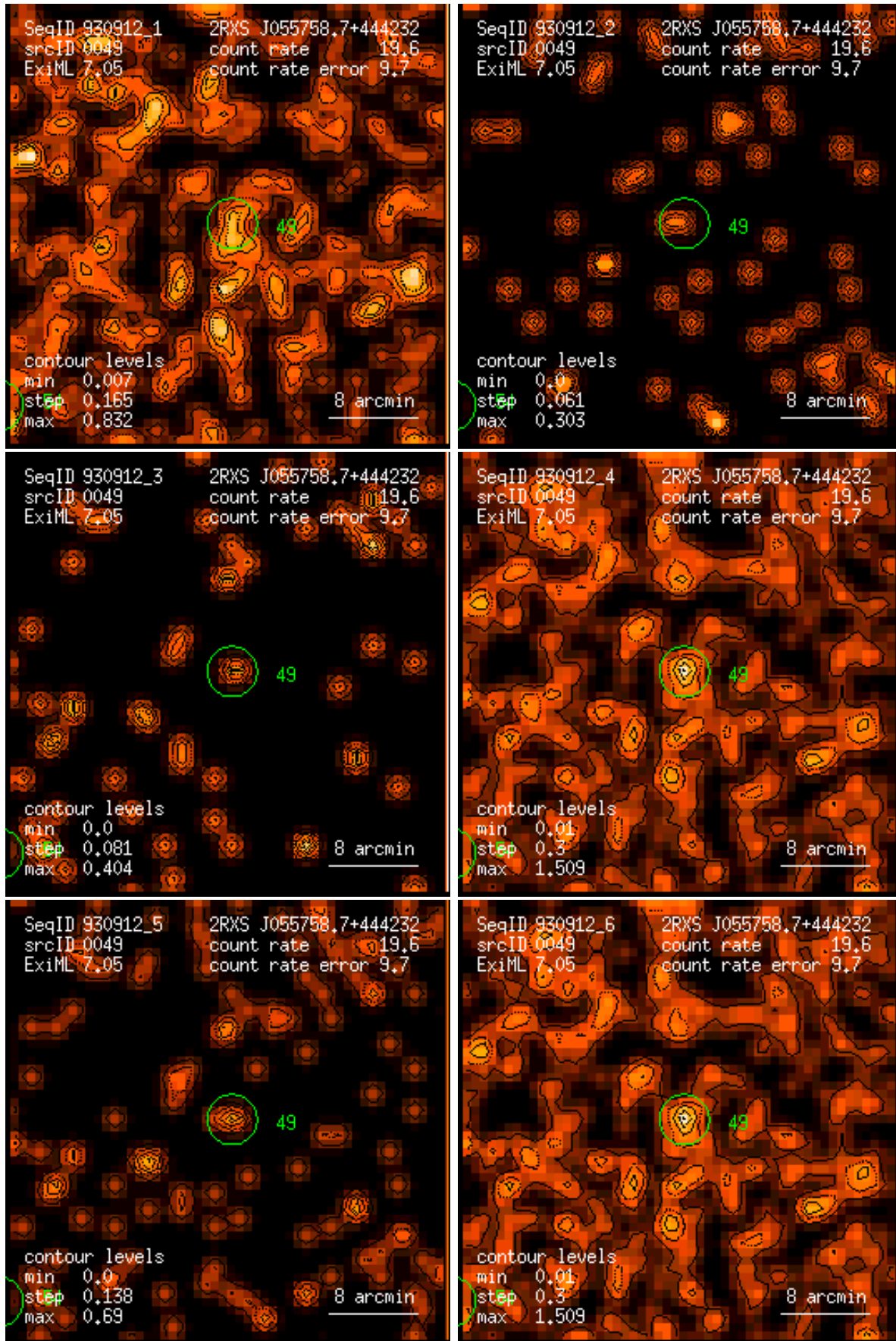
Figure 49: RASS 930912: detection 0049: band rate images, Gaussian filter: (1) PSPC channels 11 – 41, (2) 52 – 90, (3) 91 – 201, (4) 11 – 235, (5) 52 – 201, (6) 11 – 201. Broad band rates in counts/ks. Band rate contour levels in counts/ks/arcmin 2 .
