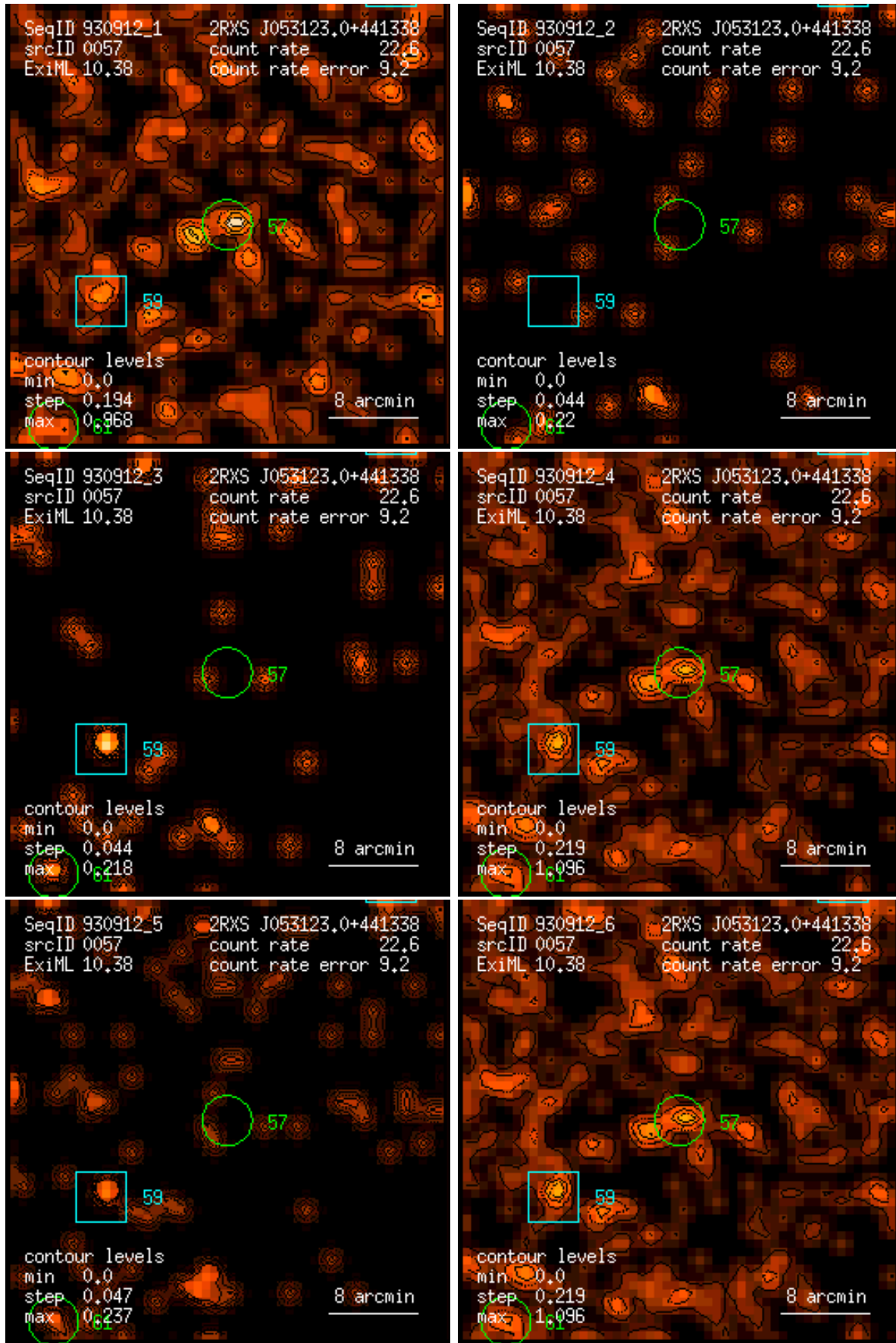
Figure 57: RASS 930912: detection 0057: band rate images, Gaussian filter: (1) PSPC channels 11 – 41, (2) 52 – 90, (3) 91 – 201, (4) 11 – 235, (5) 52 – 201, (6) 11 – 201. Broad band rates in counts/ks. Band rate contour levels in counts/ks/arcmin 2 .
