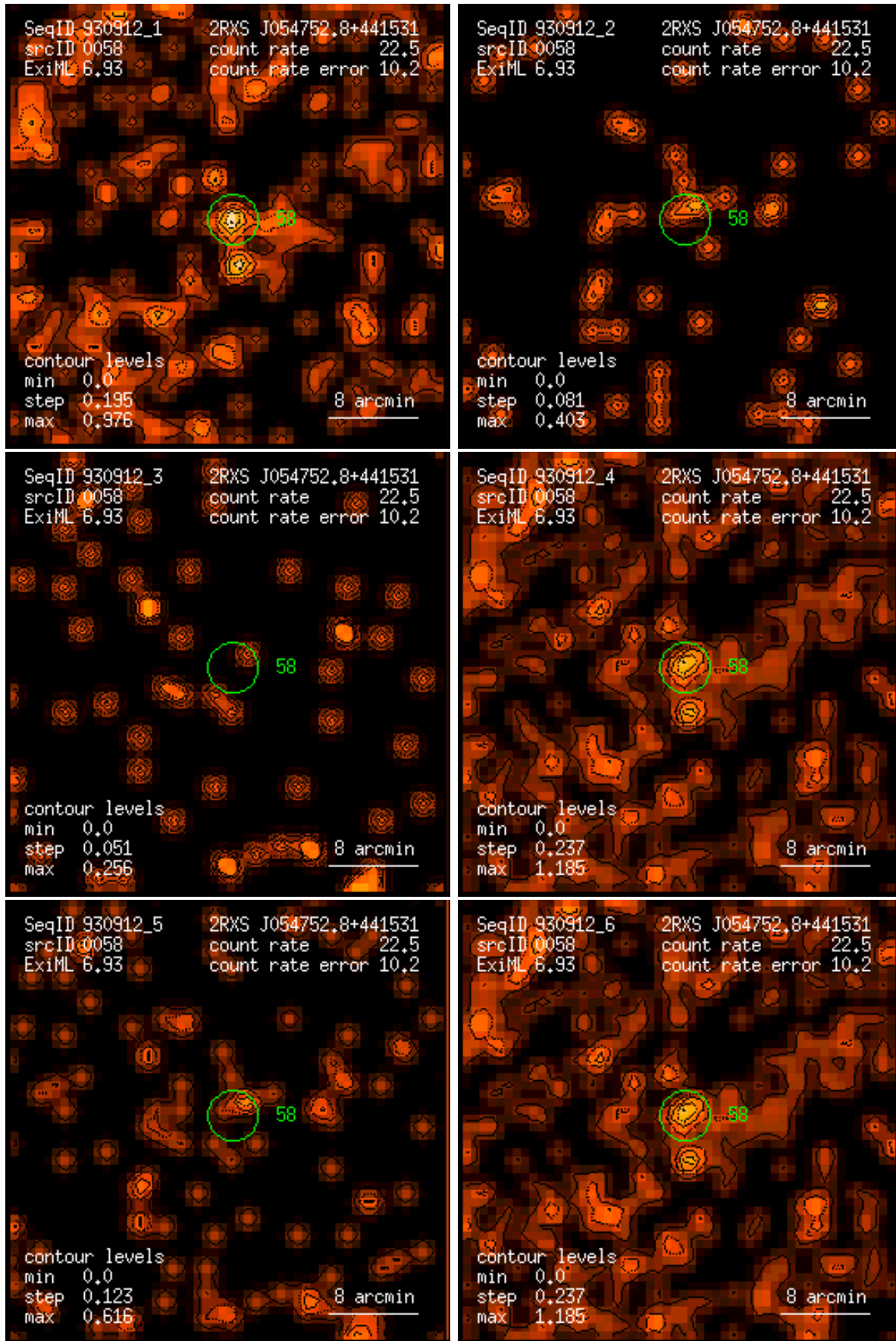
Figure 58: RASS 930912: detection 0058: band rate images, Gaussian filter: (1) PSPC channels 11 – 41, (2) 52 – 90, (3) 91 – 201, (4) 11 – 235, (5) 52 – 201, (6) 11 – 201. Broad band rates in counts/ks. Band rate contour levels in counts/ks/arcmin 2 .
