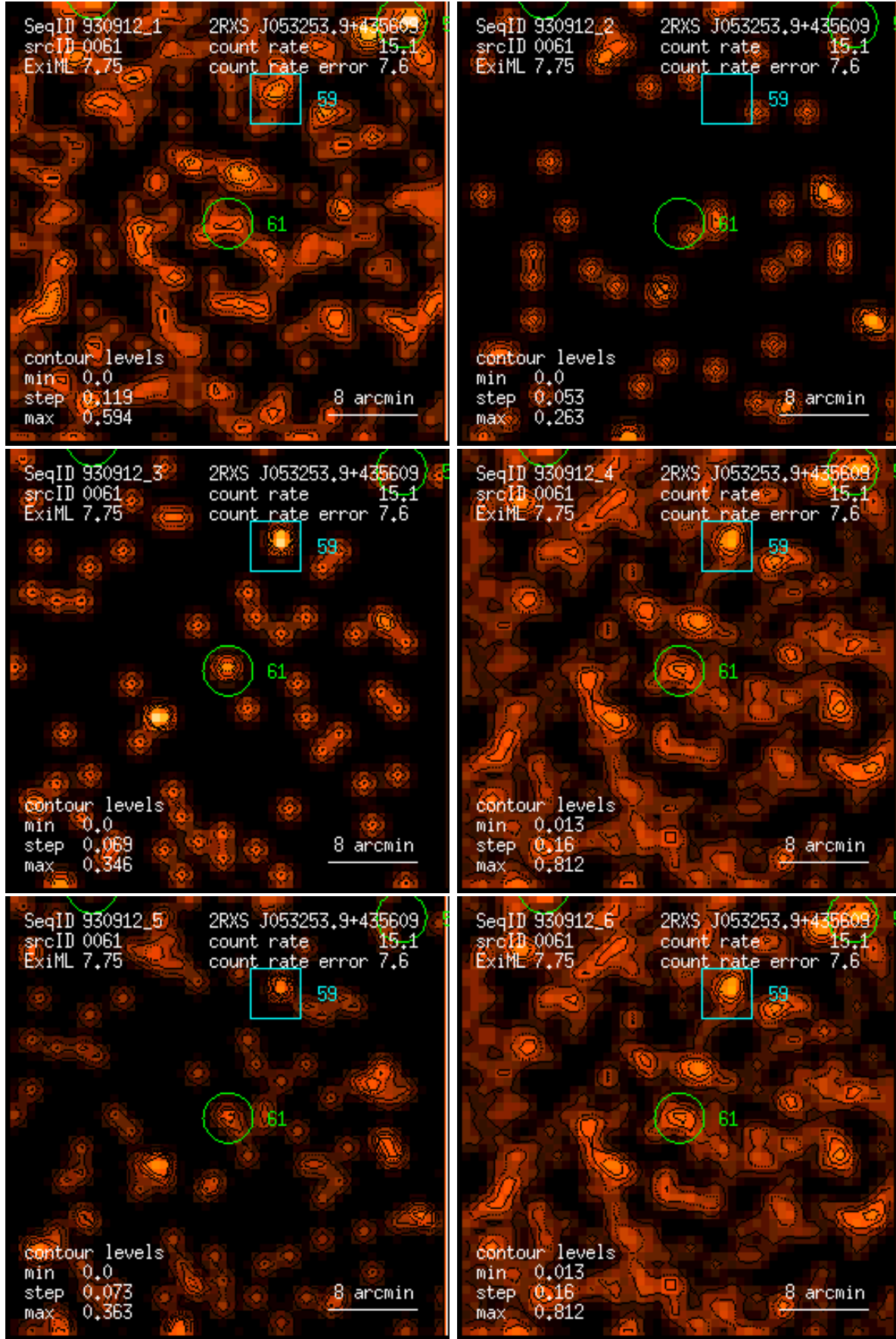
Figure 61: RASS 930912: detection 0061: band rate images, Gaussian filter: (1) PSPC channels 11 – 41, (2) 52 – 90, (3) 91 – 201, (4) 11 – 235, (5) 52 – 201, (6) 11 – 201. Broad band rates in counts/ks. Band rate contour levels in counts/ks/arcmin 2 .
