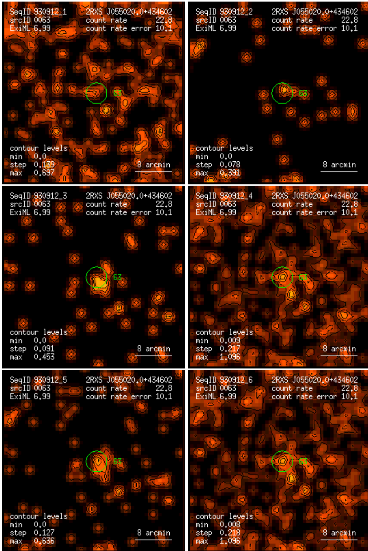
Figure 63: RASS 930912: detection 0063: band rate images, Gaussian filter: (1) PSPC channels 11 – 41, (2) 52 – 90, (3) 91 – 201, (4) 11 – 235, (5) 52 – 201, (6) 11 – 201. Broad band rates in counts/ks. Band rate contour levels in counts/ks/arcmin 2 .
