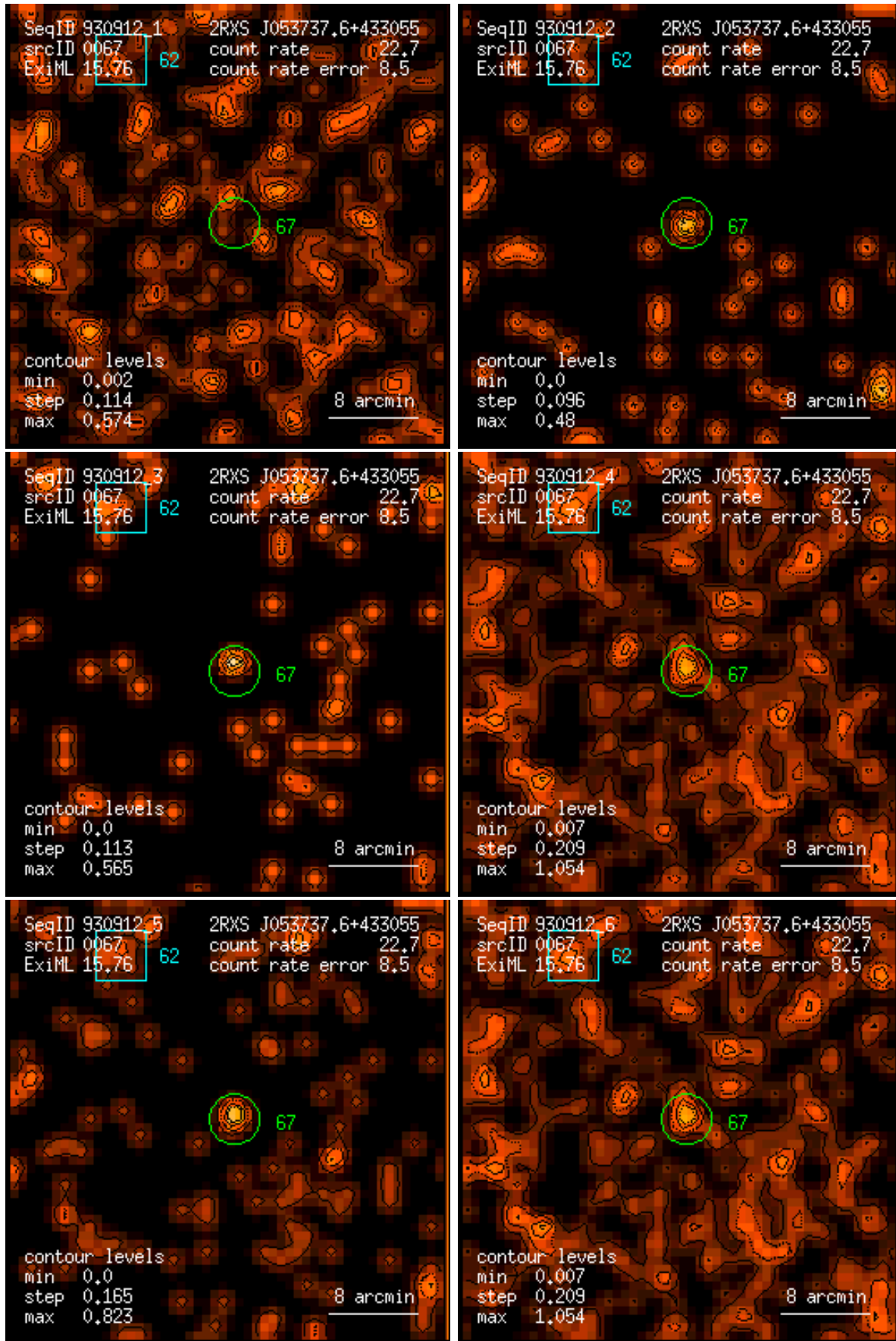
Figure 67: RASS 930912: detection 0067: band rate images, Gaussian filter: (1) PSPC channels 11 – 41, (2) 52 – 90, (3) 91 – 201, (4) 11 – 235, (5) 52 – 201, (6) 11 – 201. Broad band rates in counts/ks. Band rate contour levels in counts/ks/arcmin 2 .
