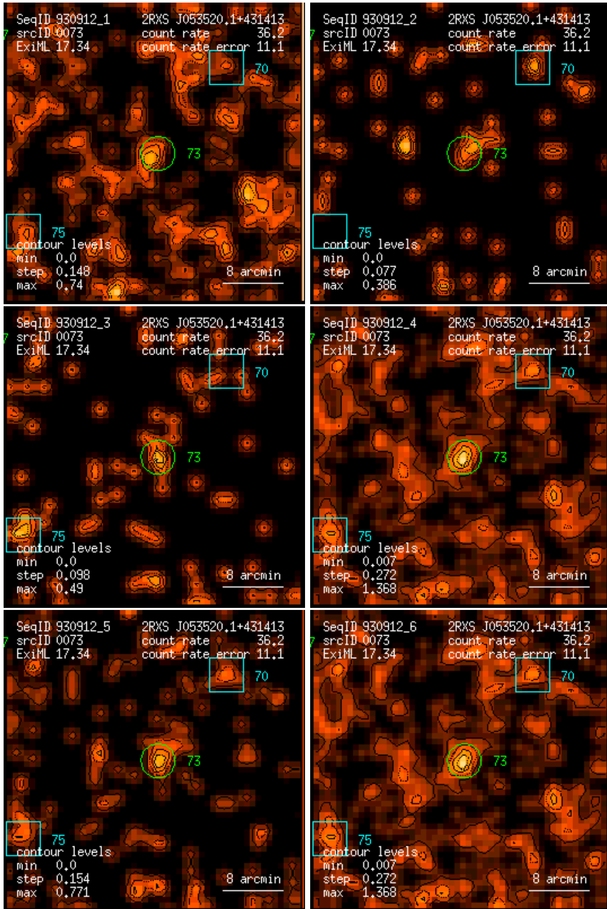
Figure 73: RASS 930912: detection 0073: band rate images, Gaussian filter: (1) PSPC channels 11 – 41, (2) 52 – 90, (3) 91 – 201, (4) 11 – 235, (5) 52 – 201, (6) 11 – 201. Broad band rates in counts/ks. Band rate contour levels in counts/ks/arcmin 2 .
