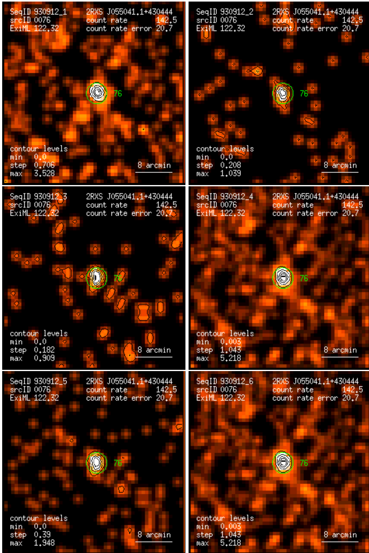
Figure 76: RASS 930912: detection 0076: band rate images, Gaussian filter: (1) PSPC channels 11 – 41, (2) 52 – 90, (3) 91 – 201, (4) 11 – 235, (5) 52 – 201, (6) 11 – 201. Broad band rates in counts/ks. Band rate contour levels in counts/ks/arcmin 2 .
