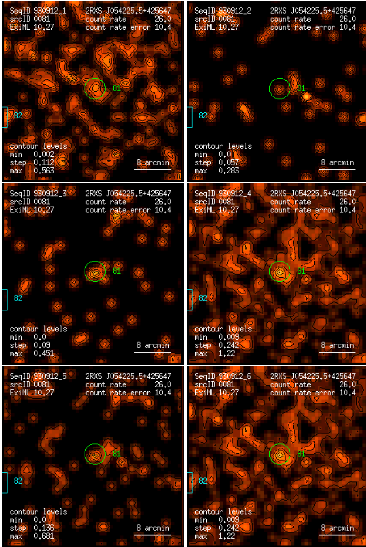
Figure 81: RASS 930912: detection 0081: band rate images, Gaussian filter: (1) PSPC channels 11 – 41, (2) 52 – 90, (3) 91 – 201, (4) 11 – 235, (5) 52 – 201, (6) 11 – 201. Broad band rates in counts/ks. Band rate contour levels in counts/ks/arcmin 2 .
