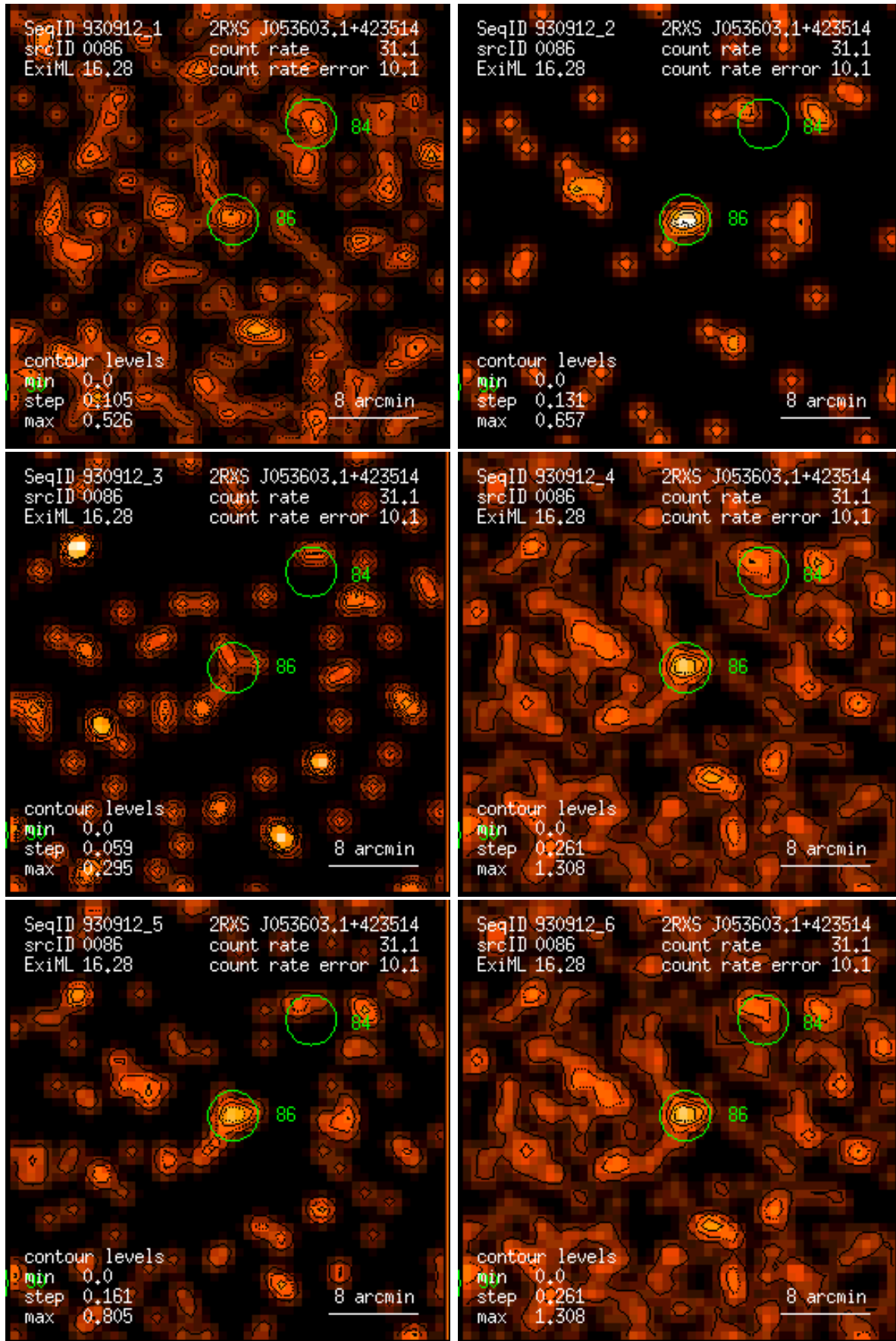
Figure 86: RASS 930912: detection 0086: band rate images, Gaussian filter: (1) PSPC channels 11 – 41, (2) 52 – 90, (3) 91 – 201, (4) 11 – 235, (5) 52 – 201, (6) 11 – 201. Broad band rates in counts/ks. Band rate contour levels in counts/ks/arcmin 2 .
