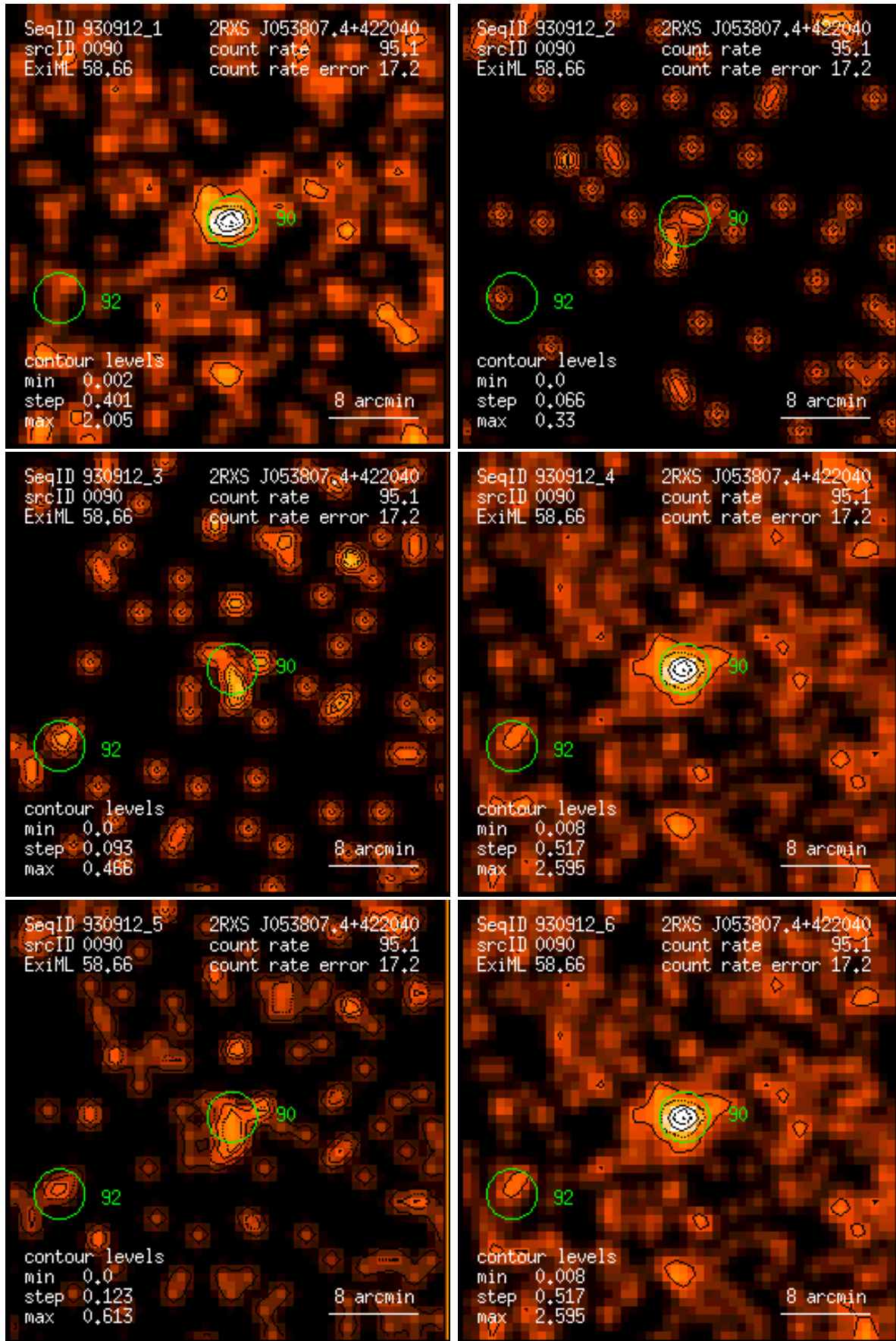
Figure 90: RASS 930912: detection 0090: band rate images, Gaussian filter: (1) PSPC channels 11 – 41, (2) 52 – 90, (3) 91 – 201, (4) 11 – 235, (5) 52 – 201, (6) 11 – 201. Broad band rates in counts/ks. Band rate contour levels in counts/ks/arcmin 2 .
