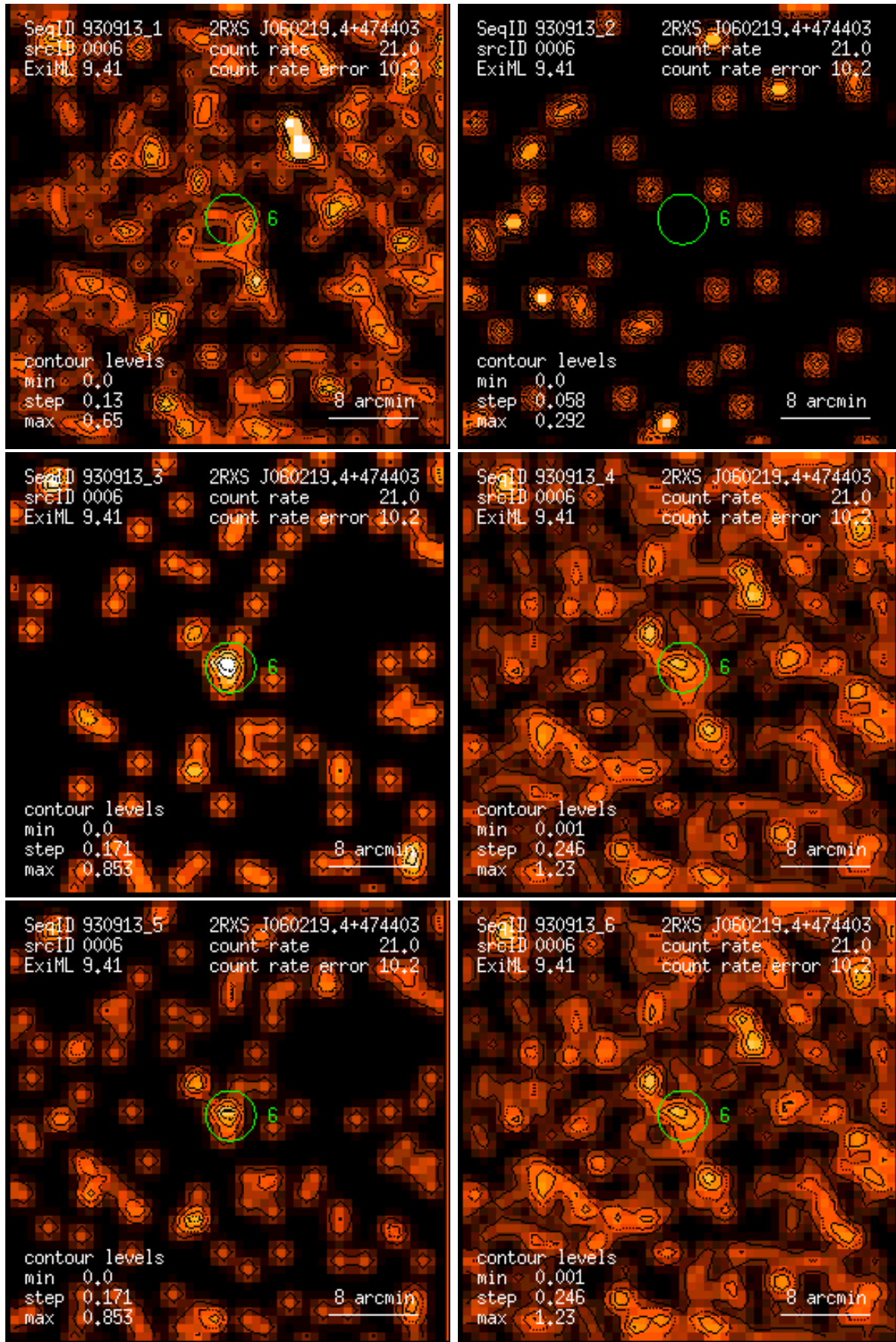
Figure 6: RASS 930913: detection 0006: band rate images, Gaussian filter: (1) PSPC channels 11 – 41, (2) 52 – 90, (3) 91 – 201, (4) 11 – 235, (5) 52 – 201, (6) 11 – 201. Broad band rates in counts/ks. Band rate contour levels in counts/ks/arcmin 2 .
