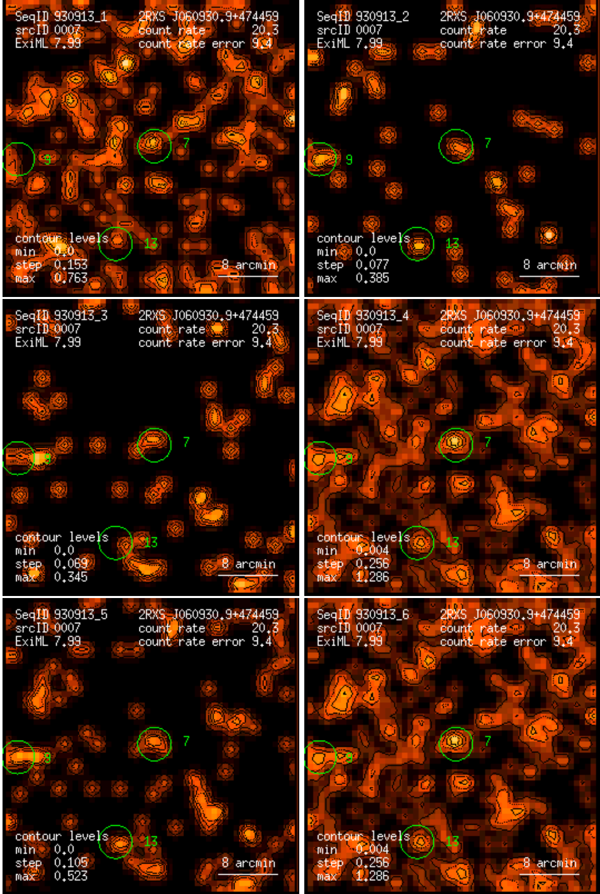
Figure 7: RASS 930913: detection 0007: band rate images, Gaussian filter: (1) PSPC channels 11 – 41, (2) 52 – 90, (3) 91 – 201, (4) 11 – 235, (5) 52 – 201, (6) 11 – 201. Broad band rates in counts/ks. Band rate contour levels in counts/ks/arcmin 2 .
