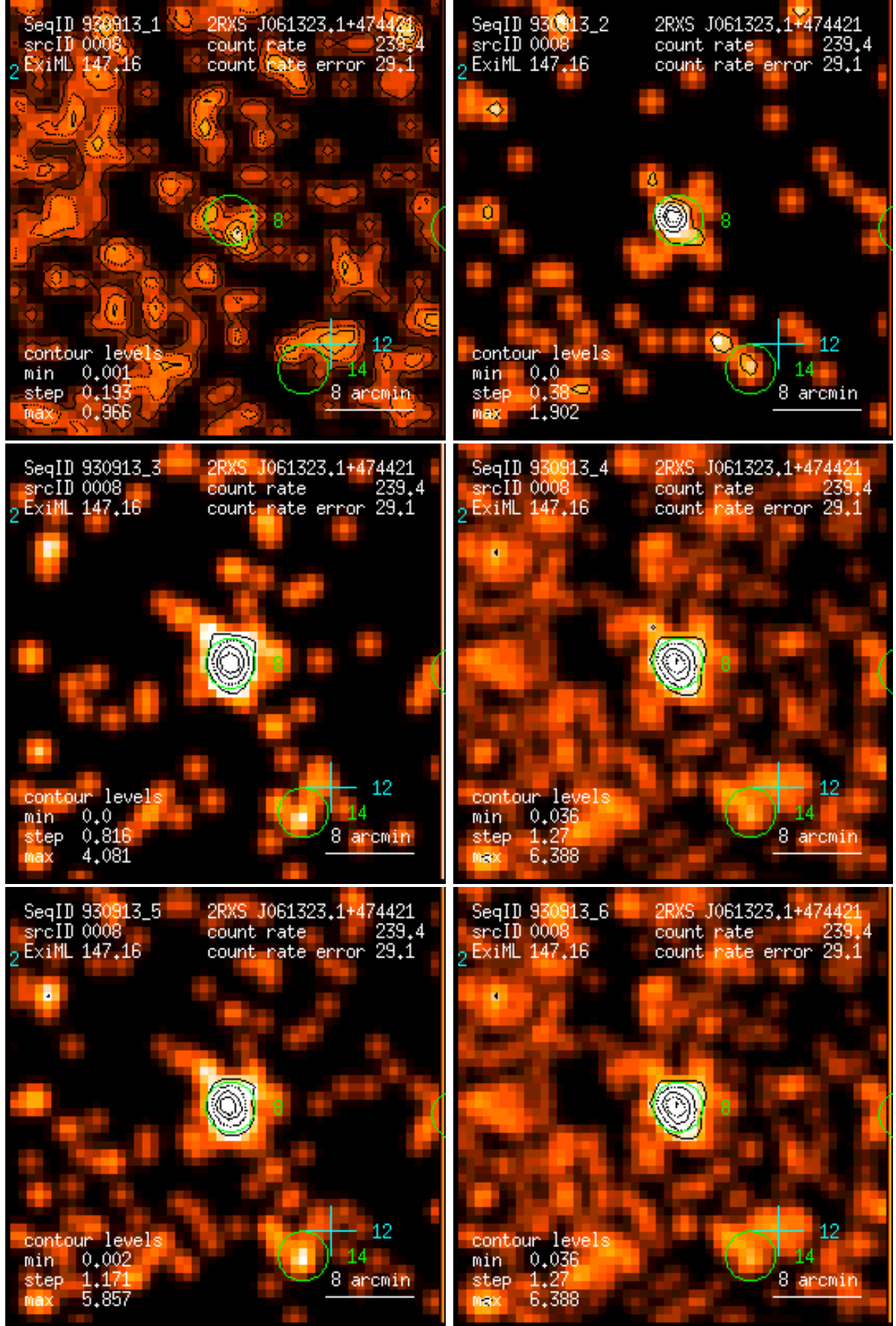
Figure 8: RASS 930913: detection 0008: band rate images, Gaussian filter: (1) PSPC channels 11 – 41, (2) 52 – 90, (3) 91 – 201, (4) 11 – 235, (5) 52 – 201, (6) 11 – 201. Broad band rates in counts/ks. Band rate contour levels in counts/ks/arcmin 2 .
