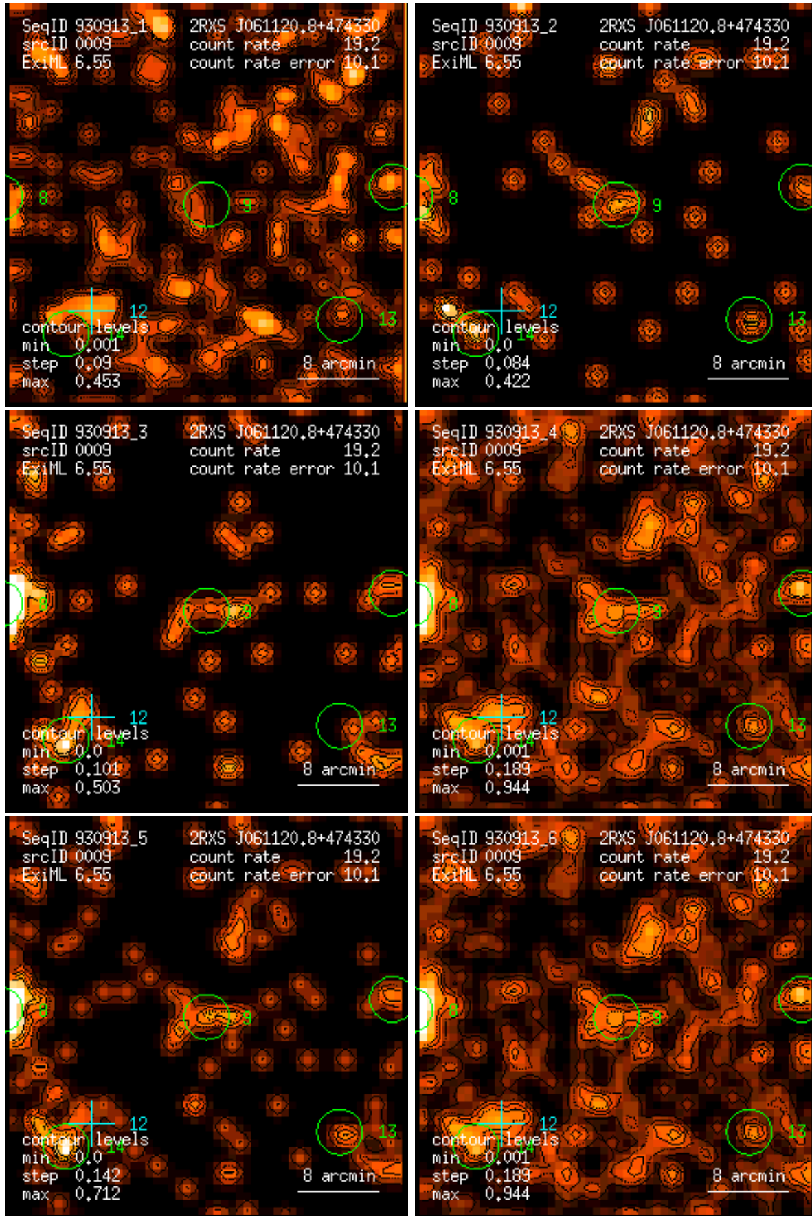
Figure 9: RASS 930913: detection 0009: band rate images, Gaussian filter: (1) PSPC channels 11 – 41, (2) 52 – 90, (3) 91 – 201, (4) 11 – 235, (5) 52 – 201, (6) 11 – 201. Broad band rates in counts/ks. Band rate contour levels in counts/ks/arcmin 2 .
