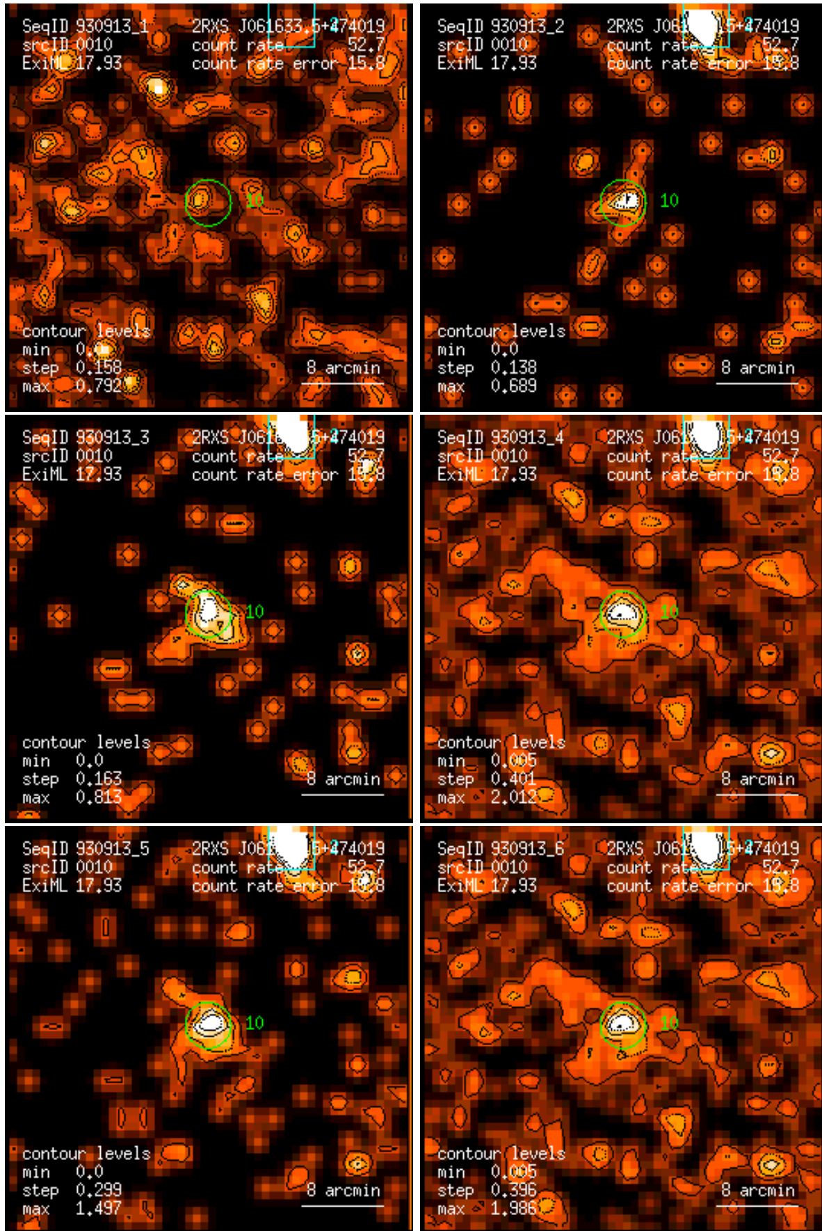
Figure 10: RASS 930913: detection 0010: band rate images, Gaussian filter: (1) PSPC channels 11 – 41, (2) 52 – 90, (3) 91 – 201, (4) 11 – 235, (5) 52 – 201, (6) 11 – 201. Broad band rates in counts/ks. Band rate contour levels in counts/ks/arcmin 2 .
