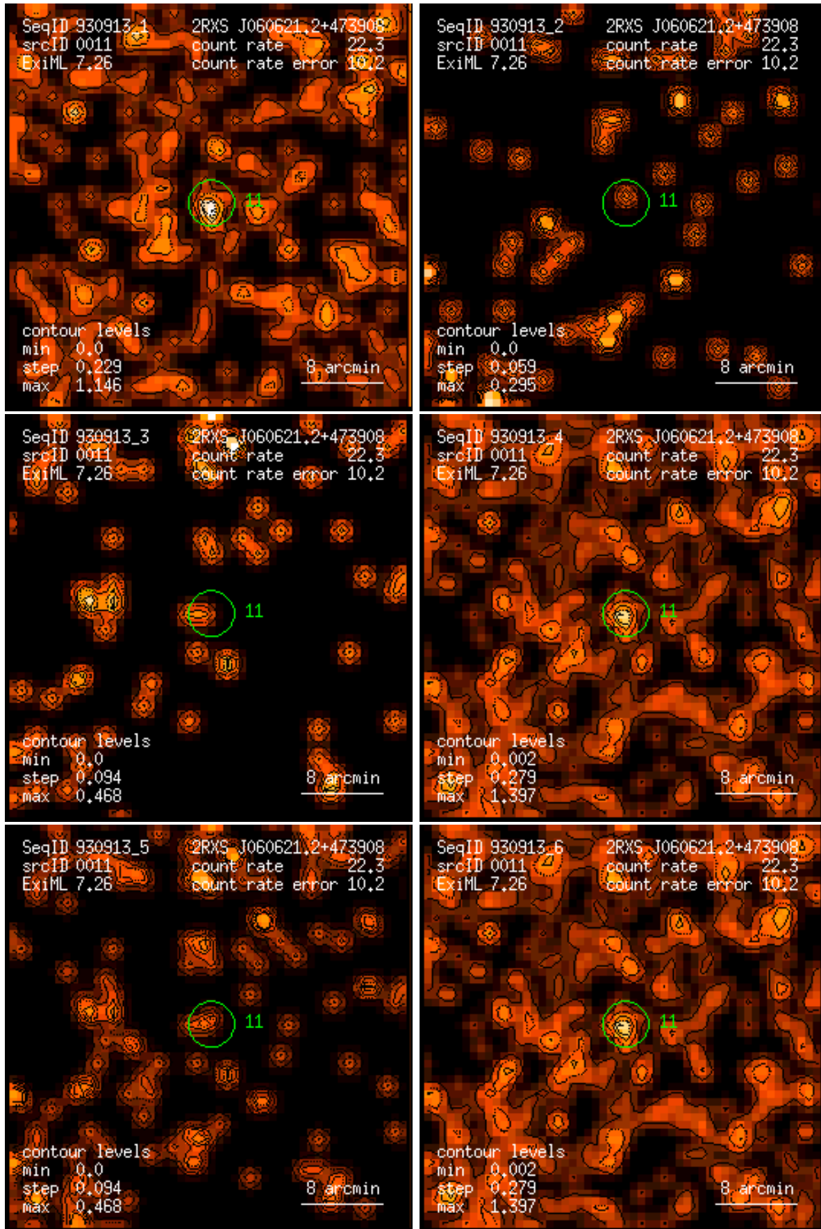
Figure 11: RASS 930913: detection 0011: band rate images, Gaussian filter: (1) PSPC channels 11 – 41, (2) 52 – 90, (3) 91 – 201, (4) 11 – 235, (5) 52 – 201, (6) 11 – 201. Broad band rates in counts/ks. Band rate contour levels in counts/ks/arcmin 2 .
