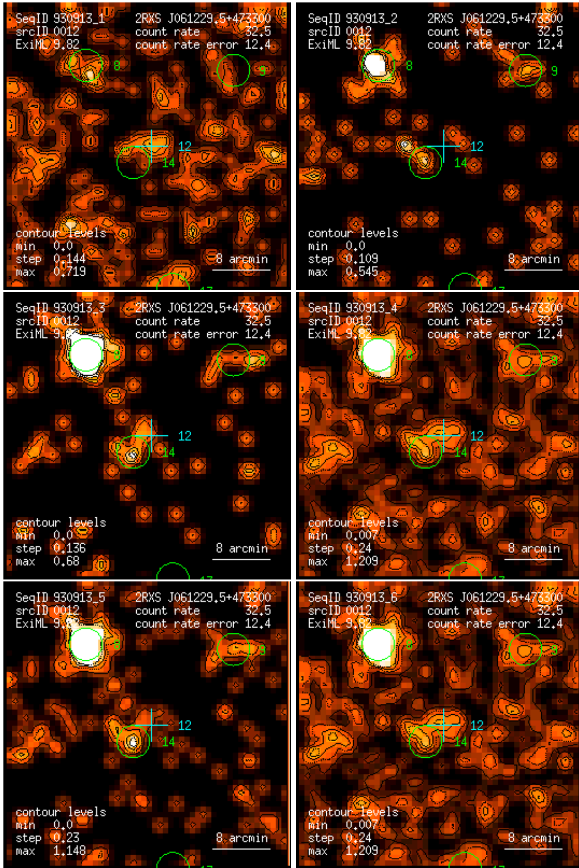
Figure 12: RASS 930913: detection 0012: band rate images, Gaussian filter: (1) PSPC channels 11 – 41, (2) 52 – 90, (3) 91 – 201, (4) 11 – 235, (5) 52 – 201, (6) 11 – 201. Broad band rates in counts/ks. Band rate contour levels in counts/ks/arcmin 2 .
