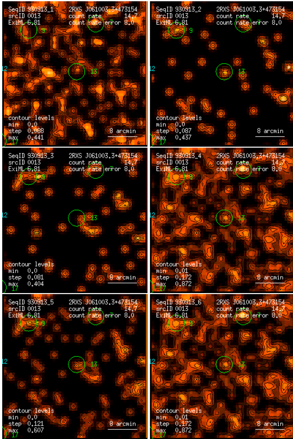
Figure 13: RASS 930913: detection 0013: band rate images, Gaussian filter: (1) PSPC channels 11 – 41, (2) 52 – 90, (3) 91 – 201, (4) 11 – 235, (5) 52 – 201, (6) 11 – 201. Broad band rates in counts/ks. Band rate contour levels in counts/ks/arcmin 2 .
