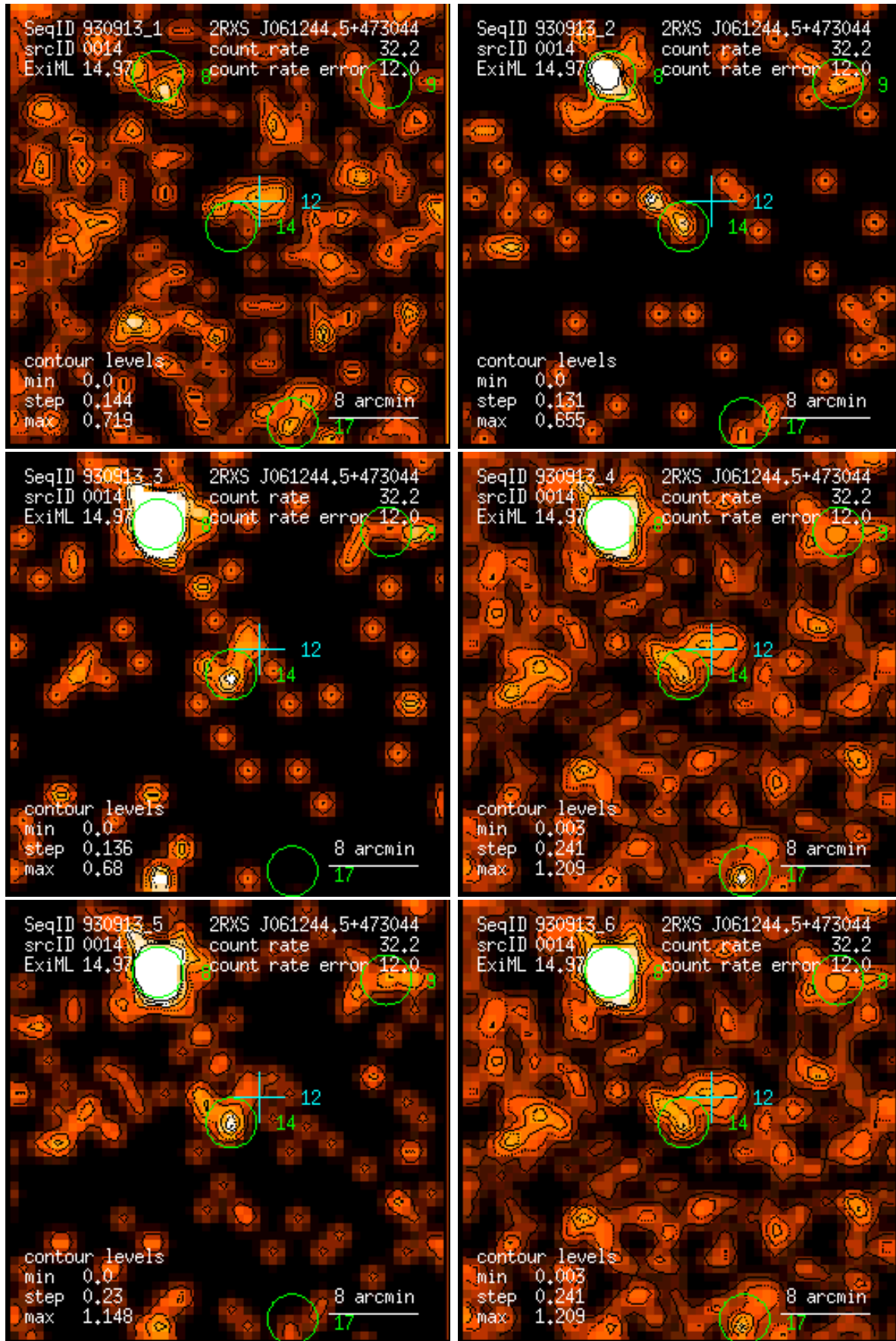
Figure 14: RASS 930913: detection 0014: band rate images, Gaussian filter: (1) PSPC channels 11 – 41, (2) 52 – 90, (3) 91 – 201, (4) 11 – 235, (5) 52 – 201, (6) 11 – 201. Broad band rates in counts/ks. Band rate contour levels in counts/ks/arcmin 2 .
