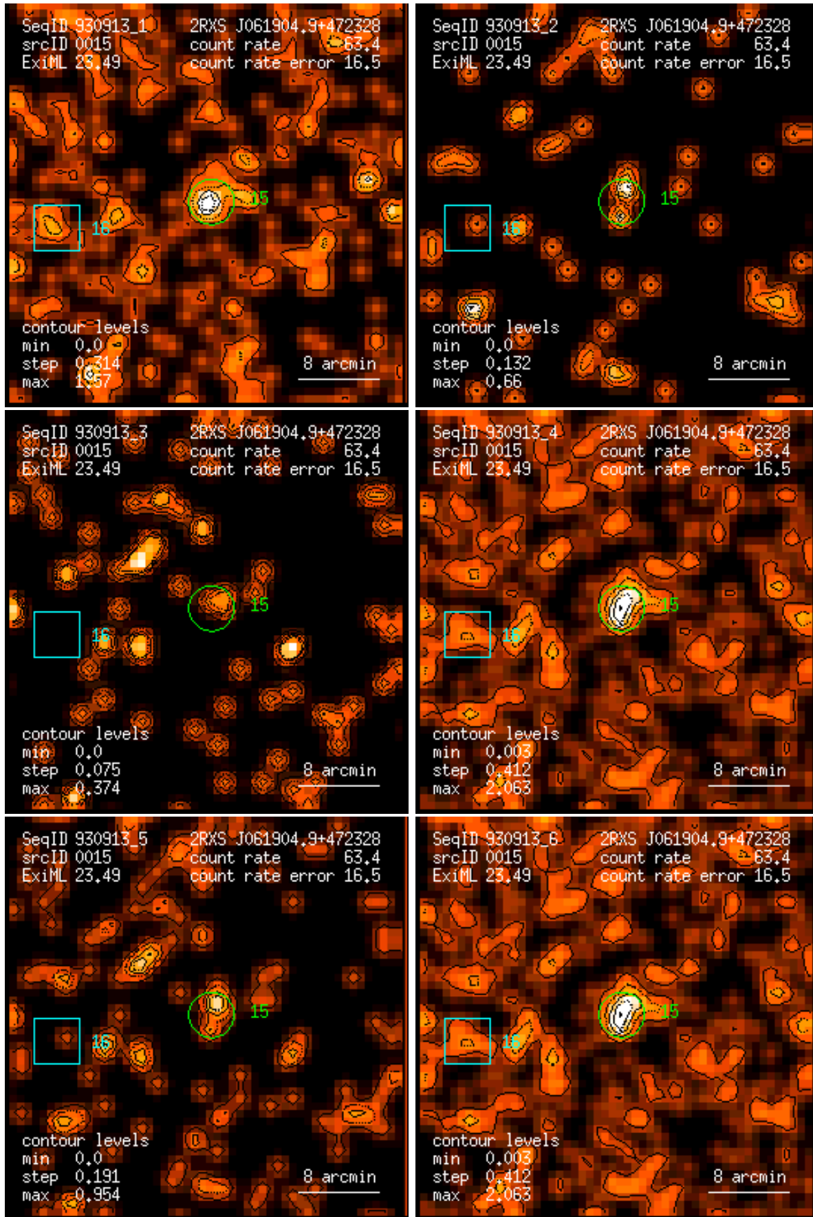
Figure 15: RASS 930913: detection 0015: band rate images, Gaussian filter: (1) PSPC channels 11 – 41, (2) 52 – 90, (3) 91 – 201, (4) 11 – 235, (5) 52 – 201, (6) 11 – 201. Broad band rates in counts/ks. Band rate contour levels in counts/ks/arcmin 2 .
